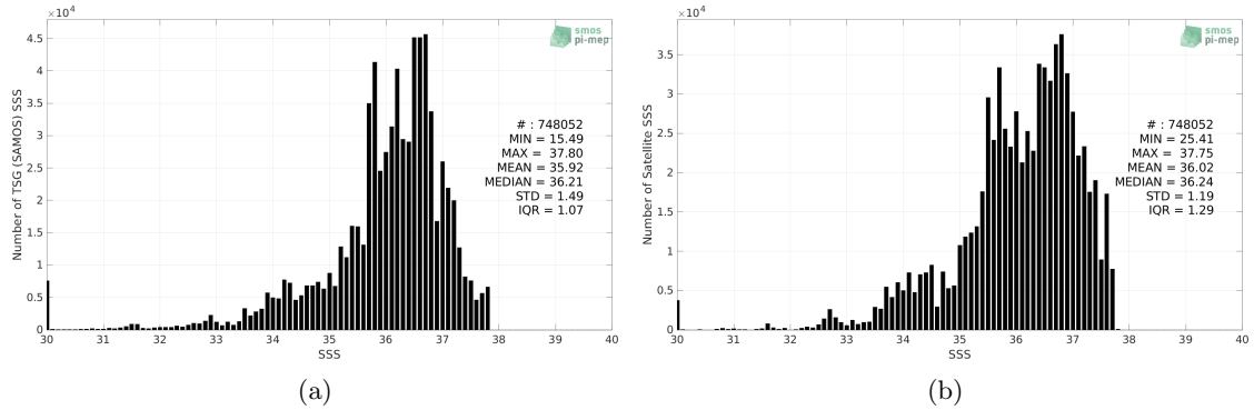
Figure 2: Histograms of SSS from TSG (SAMOS) (a) and SMAP SSS L4 OI v2 - 7 Days (ESR) (b) considering all match-up pairs per bins of 0.1 over the Amazon and Orinoco river plumes Pi-MEP region and for the full satellite product period.
