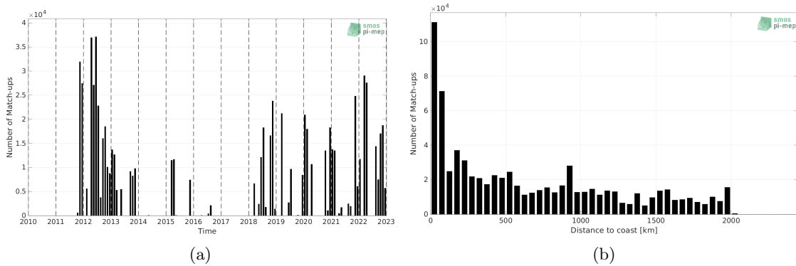
Figure 1: Number of match-ups between TSG (SAMOS) and SMAP SSS L4 OI v2 - 7 Days (ESR) SSS as a function of time (a) and as function of the distance to coast (b) over the Amazon and Orinoco river plumes Pi-MEP region and for the full satellite product period.
