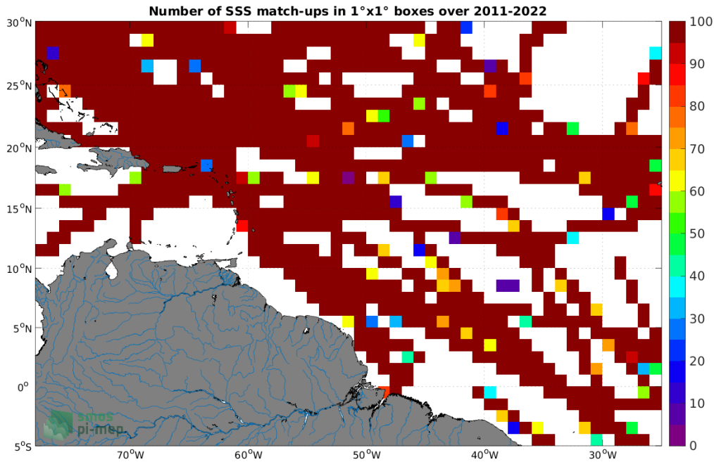
Figure 4: Number of SSS match-ups between TSG (SAMOS) SSS and the SMAP SSS L4 OI v2 - 7 Days (ESR) SSS product for the Amazon and Orinoco river plumes Pi-MEP region over 1^\circ \times 1^\circ boxes and for the full satellite product period.
