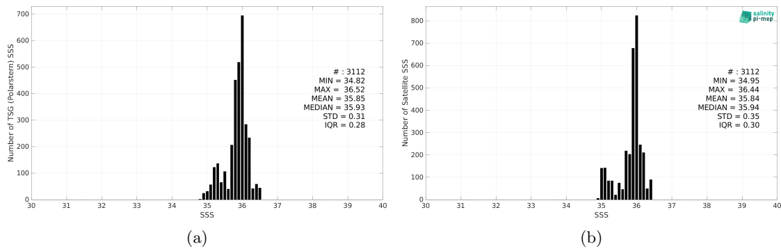
Figure 2: Histograms of SSS from TSG (Polarstern) (a) and SMAP SSS L4 OI v2 - 7 Days (ESR) (b) considering all match-up pairs per bins of 0.1 over the Amazon and Orinoco river plumes Pi-MEP region and for the full satellite product period.
