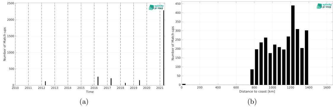
Figure 1: Number of match-ups between TSG (Polarstern) and SMAP SSS L4 OI v2 - 7 Days (ESR) SSS as a function of time (a) and as function of the distance to coast (b) over the Amazon and Orinoco river plumes Pi-MEP region and for the full satellite product period.
