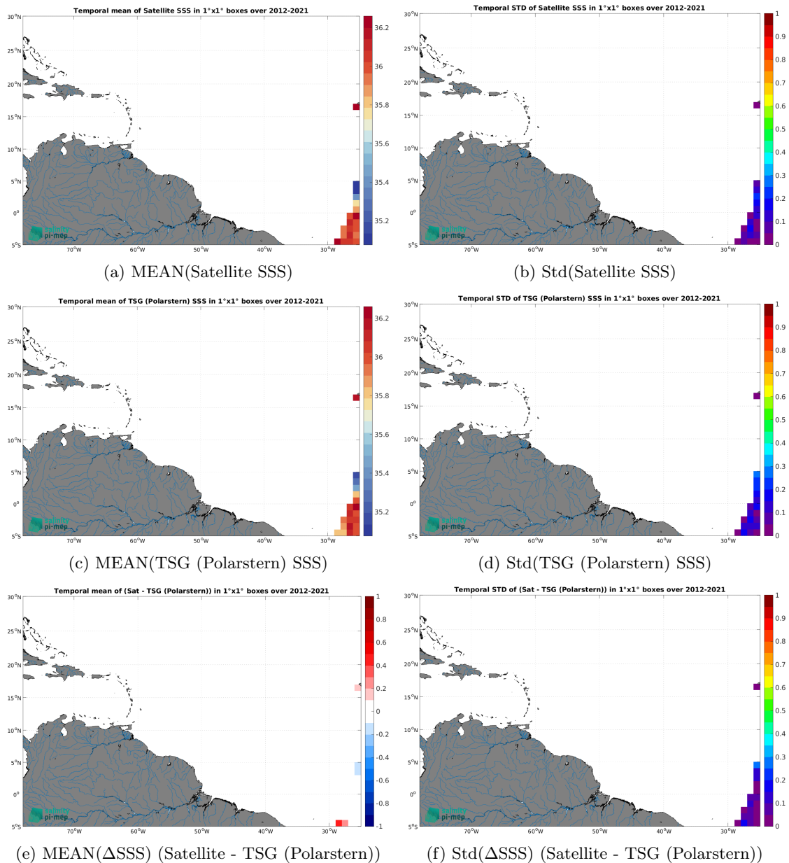
Figure 6: Temporal mean (left) and Std (right) of SSS from SMAP SSS L4 OI v2 - 7 Days (ESR) (top), TSG (Polarstern) (middle), and of \Delta SSS (Satellite - TSG (Polarstern)). Only match-up pairs are used to generate these maps.
