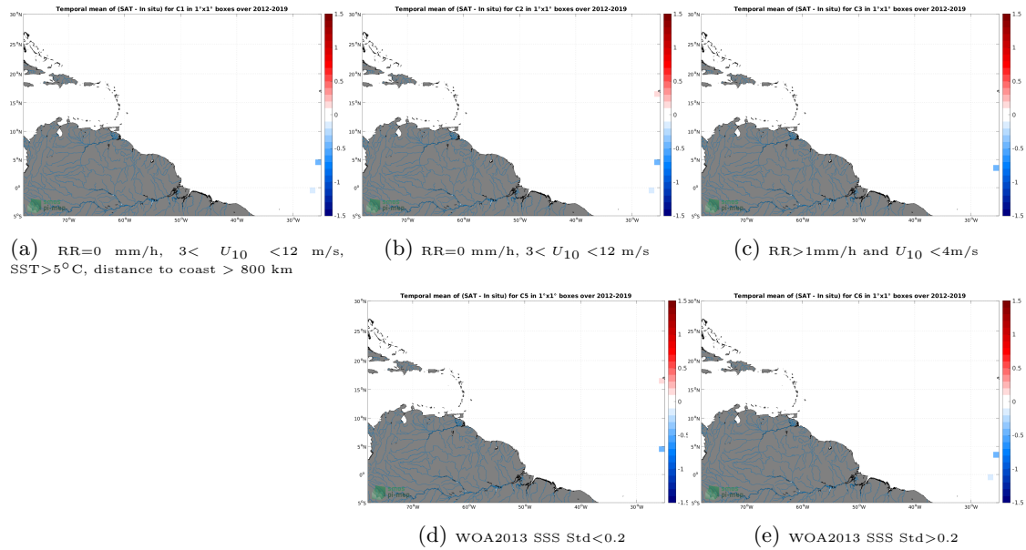
Figure 12: Temporal mean gridded over spatial boxes of size 1^\circ \times 1^\circ of \Delta SSS (SMAP SSS L4 OI v2 - 7 Days (ESR) - TSG (Polarstern)) for 5 different subdatasets corresponding to:RR=0 mm/h, 3 < U_{10} < 12 m/s, SST >5^\circ\text{C} , distance to coast > 800 km (a), RR=0 mm/h, 3 < U_{10} < 12 m/s (b), RR >1 mm/h and U_{10} < 4 m/s (c), WOA2013 SSS Std <0.2 (d), WOA2013 SSS Std >0.2 (e).
