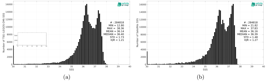
Figure 2: Histograms of SSS from TSG (LEGOS-DM) (a) and SMAP SSS L4 OI v2 - 7 Days (ESR) (b) considering all match-up pairs per bins of 0.1 over the Amazon and Orinoco river plumes Pi-MEP region and for the full satellite product period.
