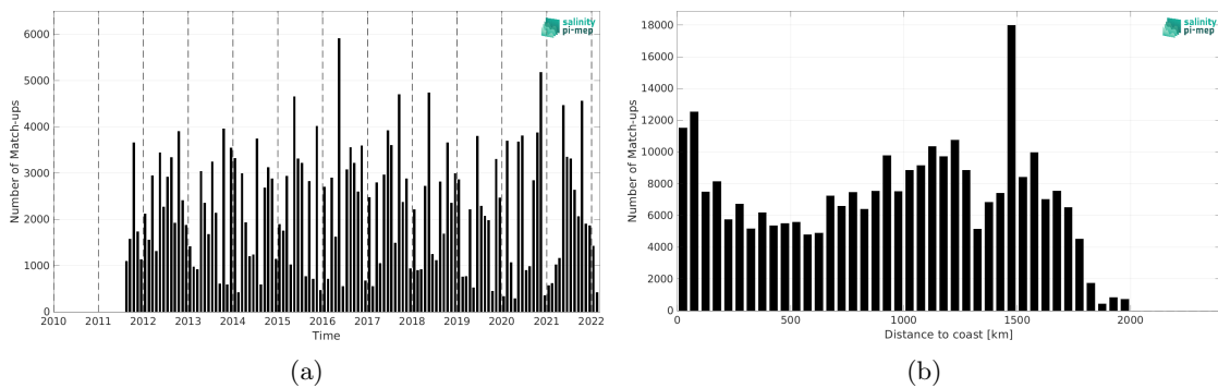
Figure 1: Number of match-ups between TSG (LEGOS-DM) and SMAP SSS L4 OI v2 - 7 Days (ESR) SSS as a function of time (a) and as function of the distance to coast (b) over the Amazon and Orinoco river plumes Pi-MEP region and for the full satellite product period.
