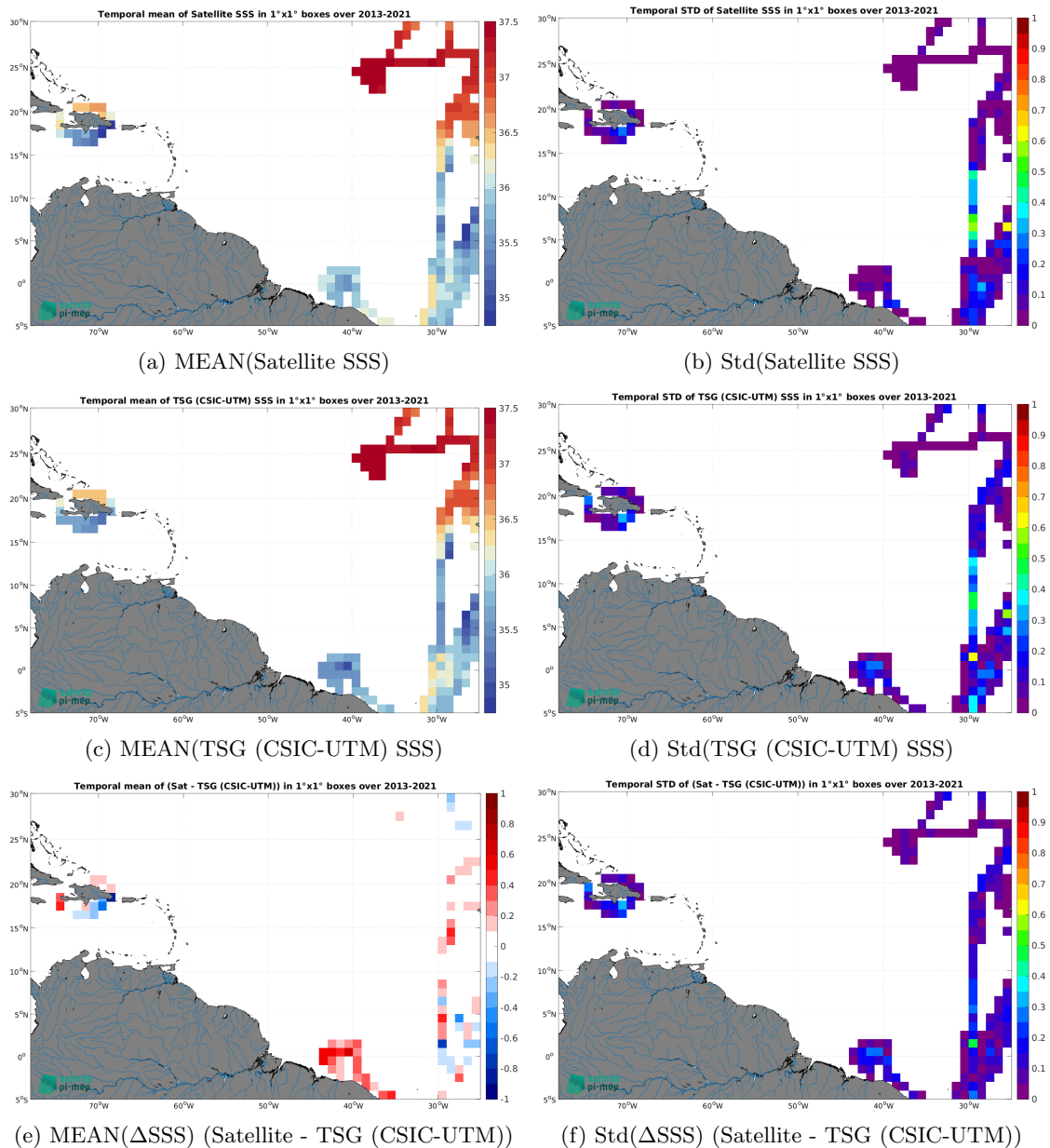
Figure 6: Temporal mean (left) and Std (right) of SSS from SMAP SSS L4 OI v2 - 7 Days (ESR) (top), TSG (CSIC-UTM) (middle), and of \Delta SSS (Satellite - TSG (CSIC-UTM)). Only match-up pairs are used to generate these maps.
