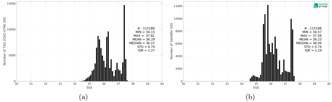
Figure 2: Histograms of SSS from TSG (CSIC-UTM) (a) and SMAP SSS L4 OI v2 - 7 Days (ESR) (b) considering all match-up pairs per bins of 0.1 over the Amazon and Orinoco river plumes Pi-MEP region and for the full satellite product period.
