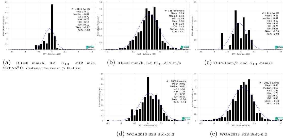
Figure 13: Normalized histogram of \Delta\text{SSS} (SMAP SSS L4 OI v2 - 7 Days (ESR) - Saldrone) for 5 different subdatasets corresponding to: RR=0 mm/h, 3 < U_{10} < 12 m/s, SST>5°C, distance to coast > 800 km (a), RR=0 mm/h, 3 < U_{10} < 12 m/s (b), RR>1mm/h and U_{10} < 4 m/s (c), WOA2013 SSS Std<0.2 (d), WOA2013 SSS Std>0.2 (e).
