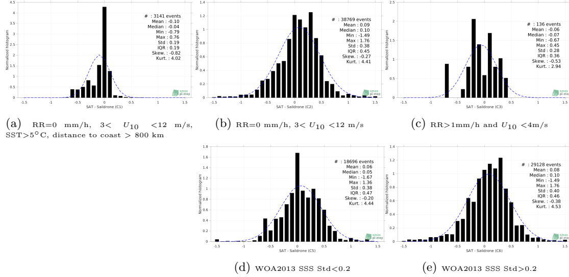
Figure 13: Normalized histogram of \Delta SSS (SMAP SSS L4 OI v2 - 7 Days (ESR) - Sairdrone) for 5 different subdatasets corresponding to: RR=0 mm/h, 3 < U_{10} < 12 m/s, SST>5°C, distance to coast > 800 km (a), RR=0 mm/h, 3 < U_{10} < 12 m/s (b), RR>1mm/h and U_{10} < 4 m/s (c), WOA2013 SSS Std<0.2 (d), WOA2013 SSS Std>0.2 (e).
