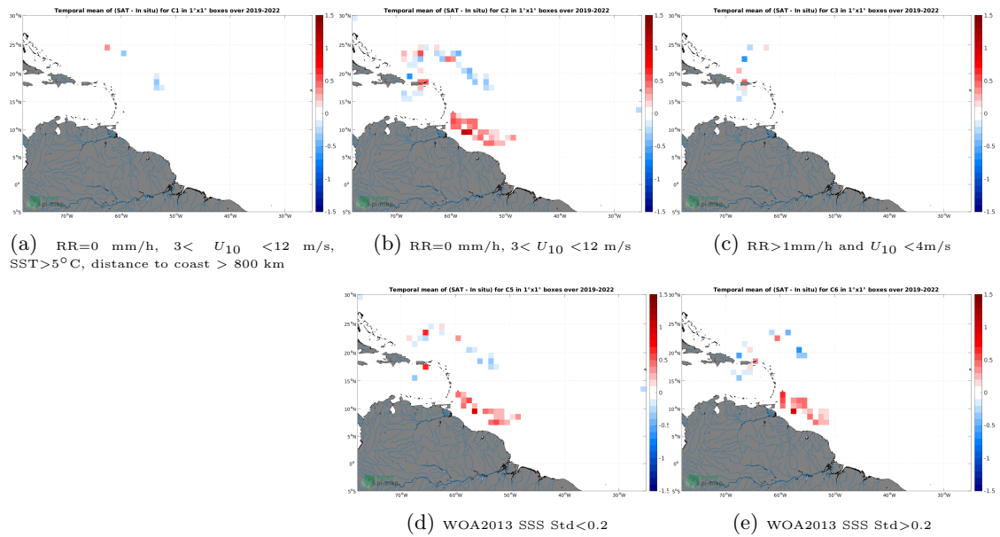
Figure 12: Temporal mean gridded over spatial boxes of size 1^\circ \times 1^\circ of \Delta SSS (SMAP SSS L4 OI v2 - 7 Days (ESR) - Saildrone) for 5 different subdatasets corresponding to:RR=0 mm/h, 3 < U_{10} < 12 m/s, SST >5^\circ\text{C} , distance to coast > 800 km (a), RR=0 mm/h, 3 < U_{10} < 12 m/s (b), RR >1 mm/h and U_{10} < 4 m/s (c), WOA2013 SSS Std <0.2 (d), WOA2013 SSS Std >0.2 (e).
