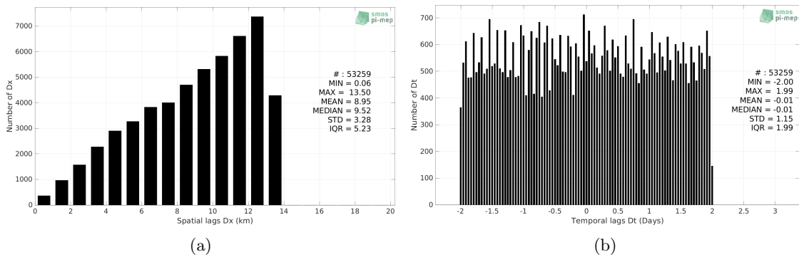
Figure 5: Histograms of the spatial (a) and temporal (b) lags between the location/time of the Saildrone measurement and the date of the corresponding SMAP SSS L4 OI v2 - 7 Days (ESR) SSS pixel.
