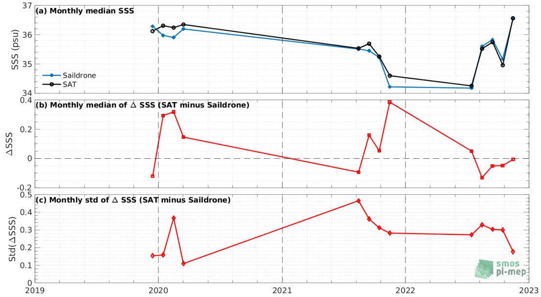
Figure 7: Time series of the monthly median SSS (top), median of \Delta\text{SSS} (Satellite - Saildrone) and Std of \Delta\text{SSS} (Satellite - Saildrone) over the Amazon and Orinoco river plumes Pi-MEP region considering all match-ups collected by the Pi-MEP.
