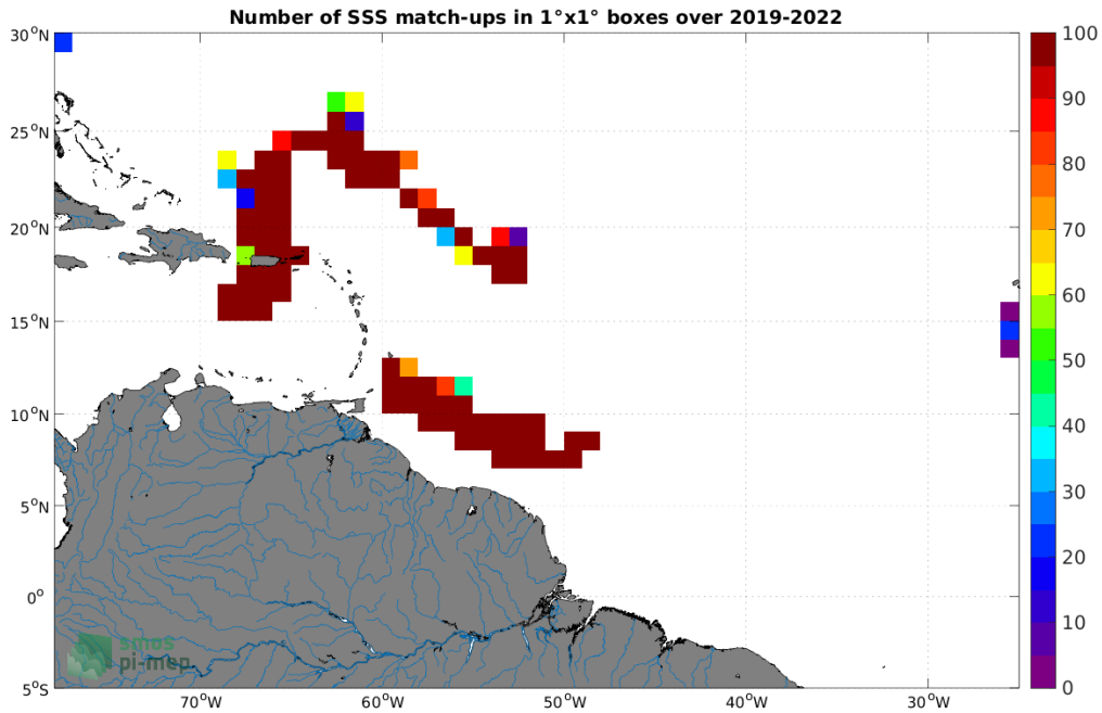
Figure 4: Number of SSS match-ups between Saildrone SSS and the SMAP SSS L4 OI v2 - 7 Days (ESR) SSS product for the Amazon and Orinoco river plumes Pi-MEP region over 1^\circ \times 1^\circ boxes and for the full satellite product period.
