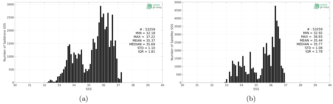
Figure 2: Histograms of SSS from Saildrone (a) and SMAP SSS L4 OI v2 - 7 Days (ESR) (b) considering all match-up pairs per bins of 0.1 over the Amazon and Orinoco river plumes Pi-MEP region and for the full satellite product period.
