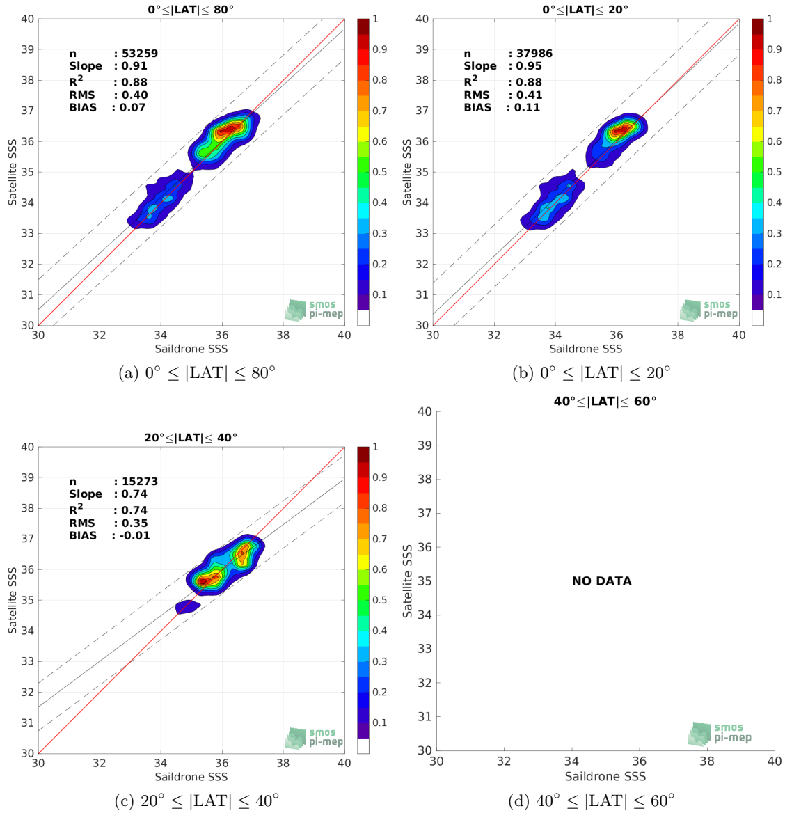
Figure 9: Contour maps of the concentration of SMAP SSS L4 OI v2 - 7 Days (ESR) SSS (y-axis) versus Saildrone SSS (x-axis) at match-up pairs for different latitude bands. For each plot, the red line shows x=y . The black thin and dashed lines indicate a linear fit through the data cloud and the \pm 95\% confidence levels, respectively. The number match-up pairs n , the slope and R^2 coefficient of the linear fit, the root mean square (RMS) and the mean bias between satellite and in situ data are indicated for each latitude band in each plots.
