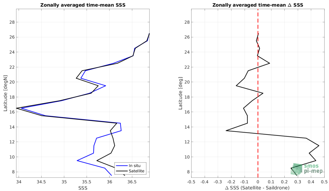
Figure 8: Left panel: Zonal mean SSS from SMAP SSS L4 OI v2 - 7 Days (ESR) satellite product (black) and from Saildrone (blue). Right panel: Zonal mean of \Delta SSS (Satellite - Saildrone) for all the collected Pi-MEP match-up pairs estimated over the full satellite product period.
