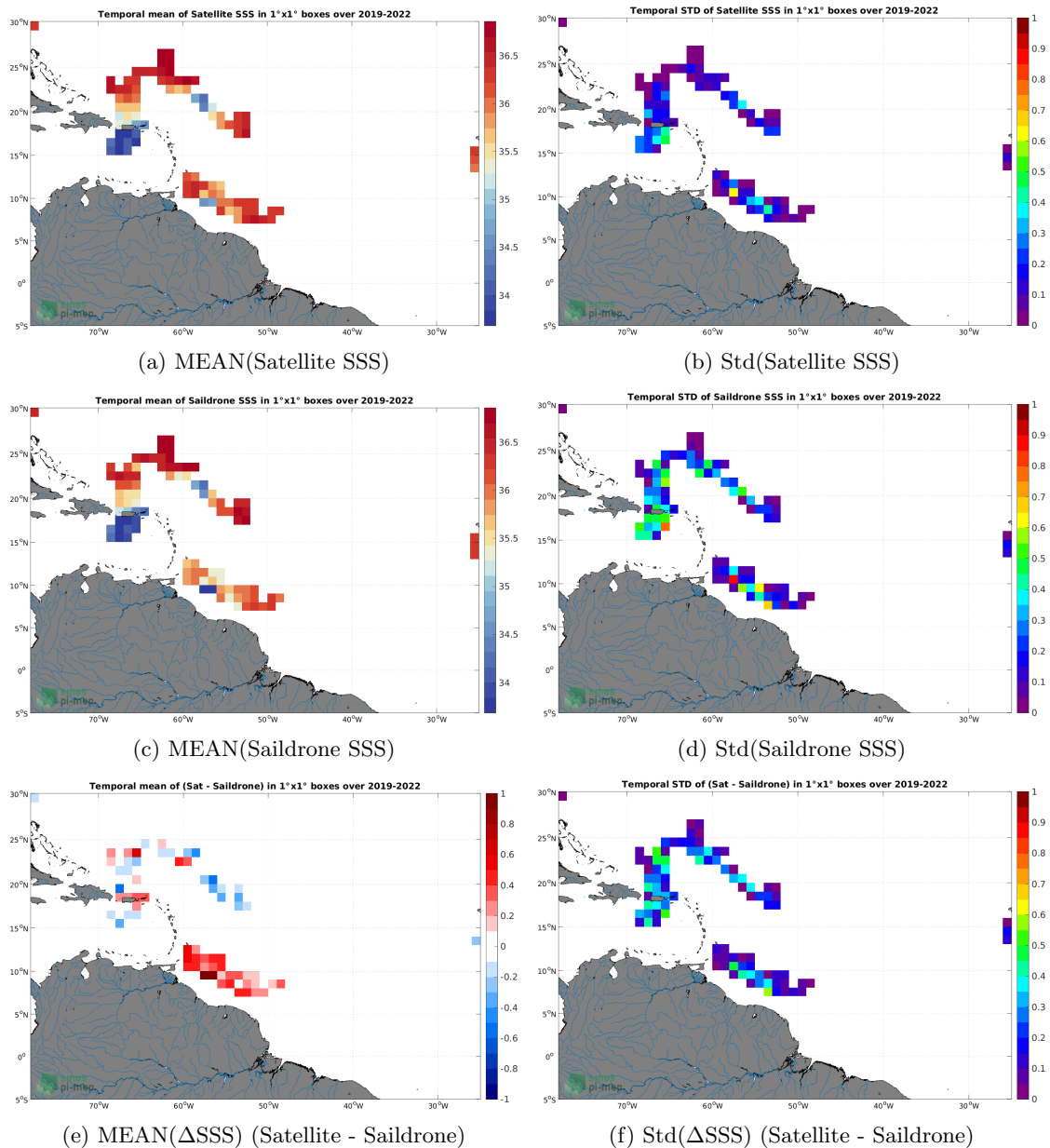
Figure 6: Temporal mean (left) and Std (right) of SSS from SMAP SSS L4 OI v2 - 7 Days (ESR) (top), Saildrone (middle), and of \Delta SSS (Satellite - Saildrone). Only match-up pairs are used to generate these maps.
