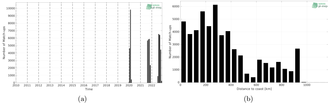
Figure 1: Number of match-ups between Saildrone and SMAP SSS L4 OI v2 - 7 Days (ESR) SSS as a function of time (a) and as function of the distance to coast (b) over the Amazon and Orinoco river plumes Pi-MEP region and for the full satellite product period.
