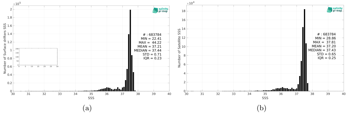
Figure 2: Histograms of SSS from Surface drifters (a) and SMAP SSS L4 OI v2 - 7 Days (ESR) (b) considering all match-up pairs per bins of 0.1 over the Amazon and Orinoco river plumes Pi-MEP region and for the full satellite product period.
