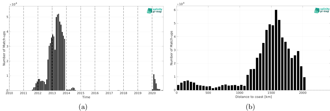
Figure 1: Number of match-ups between Surface drifters and SMAP SSS L4 OI v2 - 7 Days (ESR) SSS as a function of time (a) and as function of the distance to coast (b) over the Amazon and Orinoco river plumes Pi-MEP region and for the full satellite product period.
