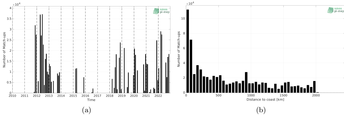
Figure 1: Number of match-ups between TSG (SAMOS) and SMAP SSS L4 OI v2 - Monthly (IPRC) SSS as a function of time (a) and as function of the distance to coast (b) over the Amazon and Orinoco river plumes Pi-MEP region and for the full satellite product period.
