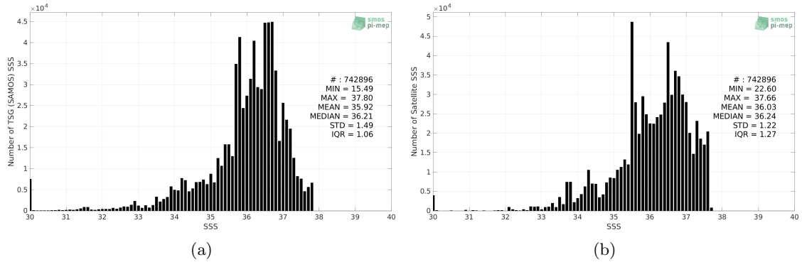
Figure 2: Histograms of SSS from TSG (SAMOS) (a) and SMAP SSS L4 OI v2 - Monthly (IPRC) (b) considering all match-up pairs per bins of 0.1 over the Amazon and Orinoco river plumes Pi-MEP region and for the full satellite product period.
