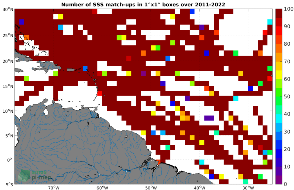
Figure 4: Number of SSS match-ups between TSG (SAMOS) SSS and the SMAP SSS L4 OI v2 - Monthly (IPRC) SSS product for the Amazon and Orinoco river plumes Pi-MEP region over 1^\circ \times 1^\circ boxes and for the full satellite product period.
