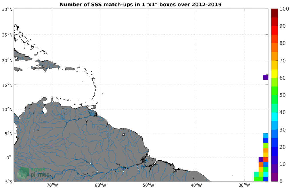
Figure 4: Number of SSS match-ups between TSG (Polarstern) SSS and the SMAP SSS L4 OI v2 - Monthly (IPRC) SSS product for the Amazon and Orinoco river plumes Pi-MEP region over 1°×1° boxes and for the full satellite product period.
