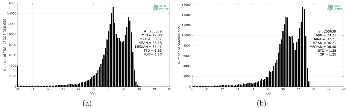
Figure 2: Histograms of SSS from TSG (LEGOS-DM) (a) and SMAP SSS L4 OI v2 - Monthly (IPRC) (b) considering all match-up pairs per bins of 0.1 over the Amazon and Orinoco river plumes Pi-MEP region and for the full satellite product period.
