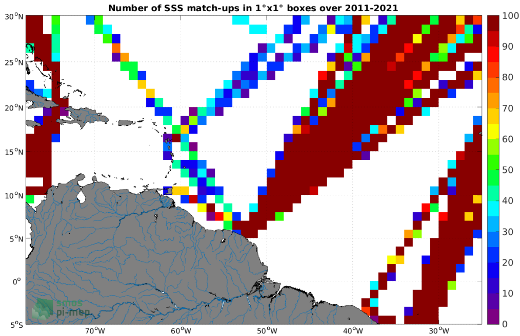
Figure 4: Number of SSS match-ups between TSG (LEGOS-DM) SSS and the SMAP SSS L4 OI v2 - Monthly (IPRC) SSS product for the Amazon and Orinoco river plumes Pi-MEP region over 1°×1° boxes and for the full satellite product period.
