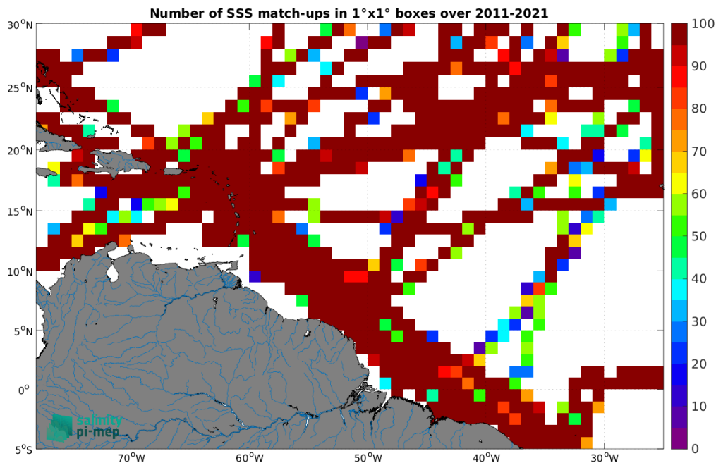
Figure 4: Number of SSS match-ups between TSG (GOSUD-Research-vessel) SSS and the SMAP SSS L4 OI v2 - Monthly (IPRC) SSS product for the Amazon and Orinoco river plumes Pi-MEP region over 1^\circ \times 1^\circ boxes and for the full satellite product period.
