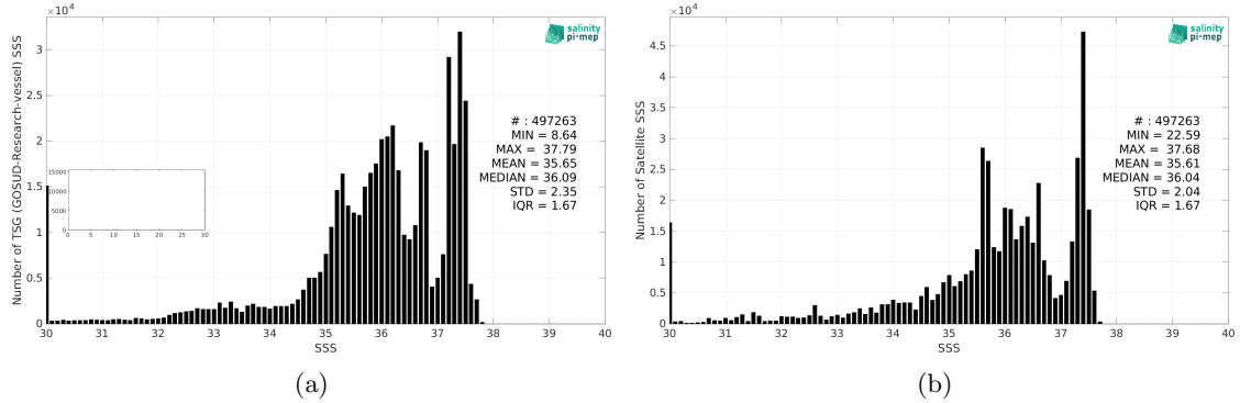
Figure 2: Histograms of SSS from TSG (GOSUD-Research-vessel) (a) and SMAP SSS L4 OI v2 - Monthly (IPRC) (b) considering all match-up pairs per bins of 0.1 over the Amazon and Orinoco river plumes Pi-MEP region and for the full satellite product period.
