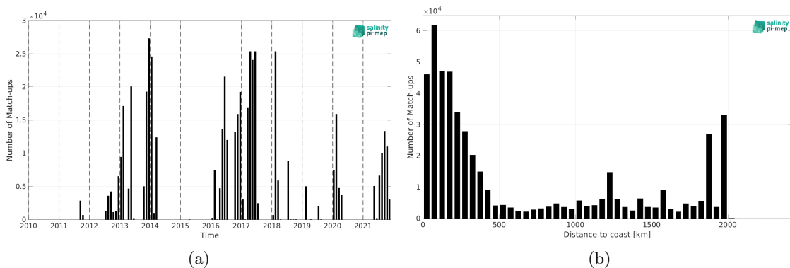
Figure 1: Number of match-ups between TSG (GOSUD-Research-vessel) and SMAP SSS L4 OI v2 - Monthly (IPRC) SSS as a function of time (a) and as function of the distance to coast (b) over the Amazon and Orinoco river plumes Pi-MEP region and for the full satellite product period.
