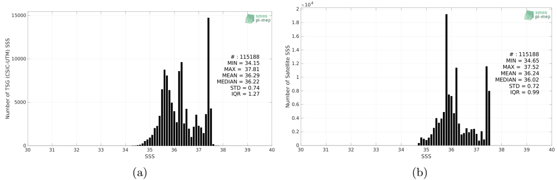
Figure 2: Histograms of SSS from TSG (CSIC-UTM) (a) and SMAP SSS L4 OI v2 - Monthly (IPRC) (b) considering all match-up pairs per bins of 0.1 over the Amazon and Orinoco river plumes Pi-MEP region and for the full satellite product period.
