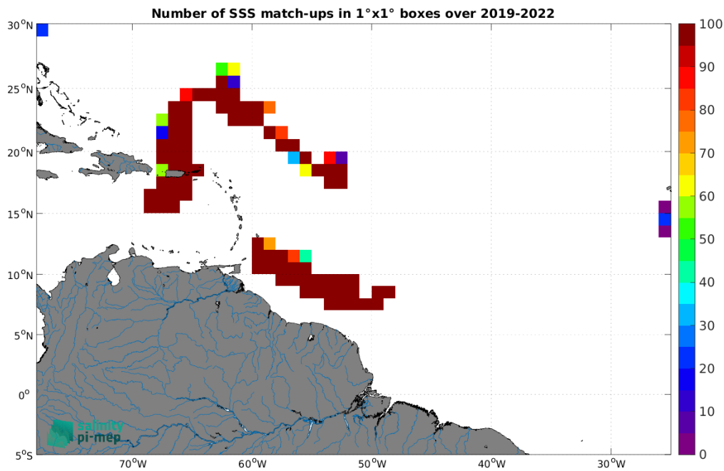
Figure 4: Number of SSS match-ups between Saildrone SSS and the SMAP SSS L4 OI v2 - Monthly (IPRC) SSS product for the Amazon and Orinoco river plumes Pi-MEP region over 1^\circ \times 1^\circ boxes and for the full satellite product period.
