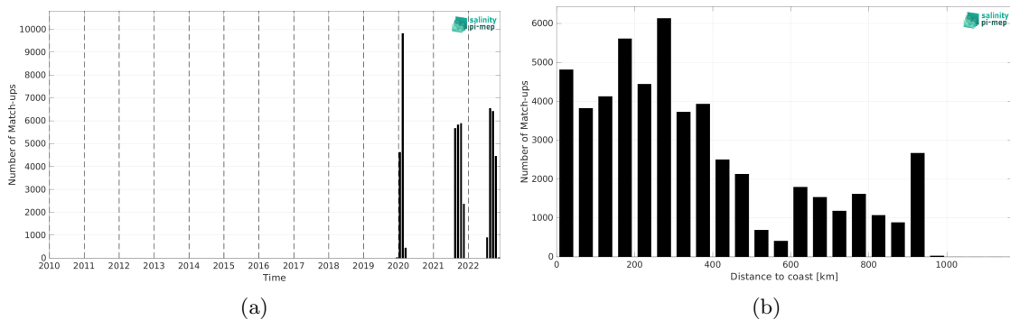
Figure 1: Number of match-ups between Saildrone and SMAP SSS L4 OI v2 - Monthly (IPRC) SSS as a function of time (a) and as function of the distance to coast (b) over the Amazon and Orinoco river plumes Pi-MEP region and for the full satellite product period.
