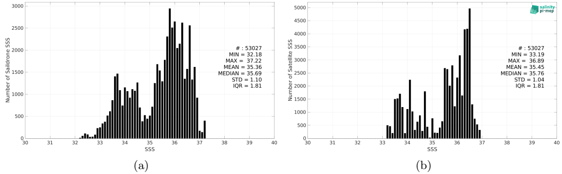
Figure 2: Histograms of SSS from Saildrone (a) and SMAP SSS L4 OI v2 - Monthly (IPRC) (b) considering all match-up pairs per bins of 0.1 over the Amazon and Orinoco river plumes Pi-MEP region and for the full satellite product period.
