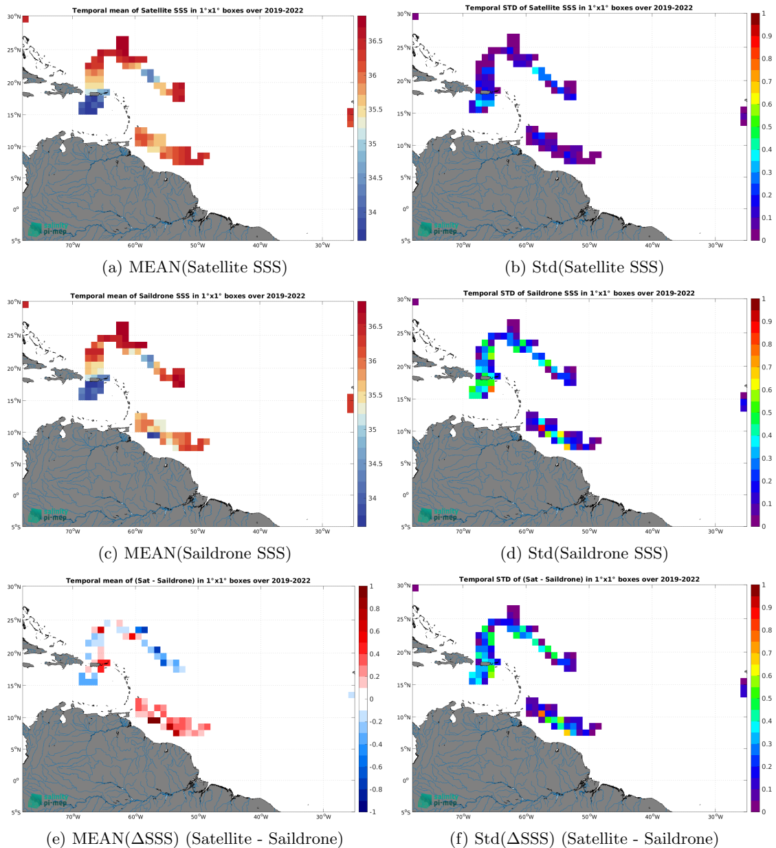
Figure 6: Temporal mean (left) and Std (right) of SSS from SMAP SSS L4 OI v2 - Monthly (IPRC) (top), Saildrone (middle), and of \Delta SSS (Satellite - Saildrone). Only match-up pairs are used to generate these maps.
