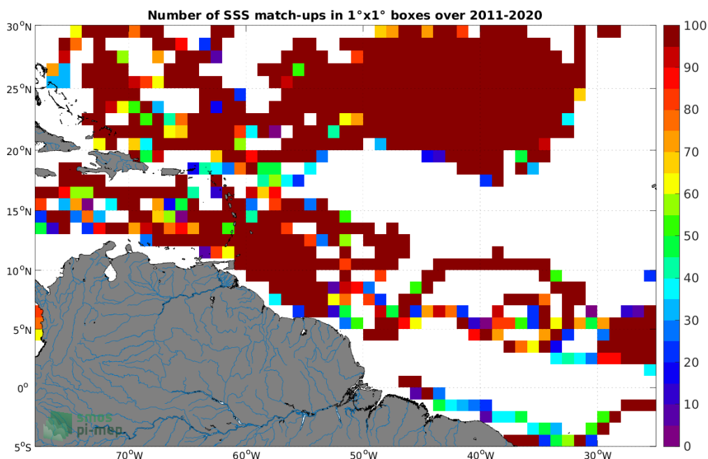
Figure 3: Number of SSS match-ups between Surface drifters SSS and the SMAP SSS L4 OI v2 - Monthly (IPRC) SSS product for the Amazon and Orinoco river plumes Pi-MEP region over 1^\circ \times 1^\circ boxes and for the full satellite product period.
