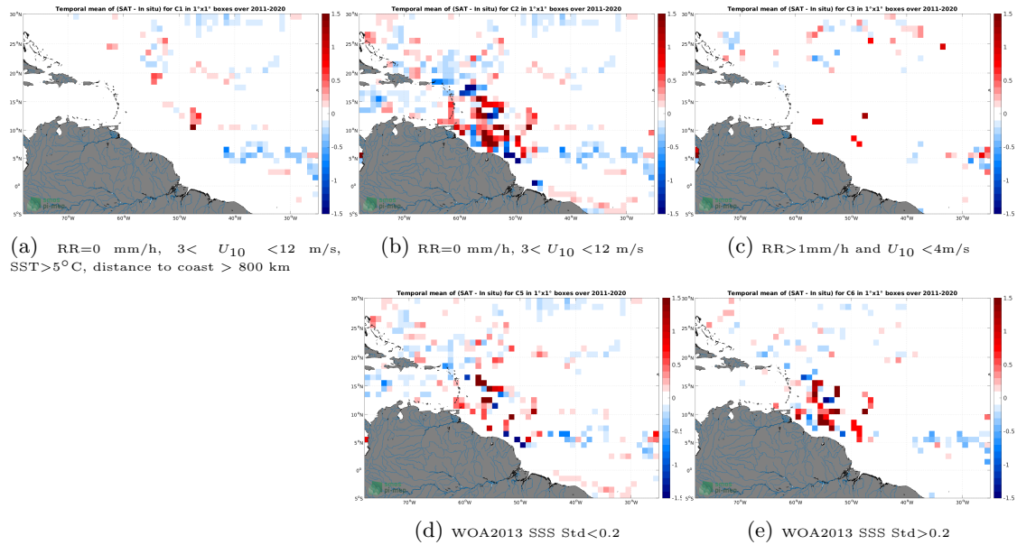
Figure 11: Temporal mean gridded over spatial boxes of size 1^\circ \times 1^\circ of \Delta SSS (SMAP SSS L4 OI v2 - Monthly (IPRC) - Surface drifters) for 5 different subdatasets corresponding to: RR=0 mm/h, 3 < U_{10} < 12 m/s, SST > 5^\circ C , distance to coast > 800 km (a), RR=0 mm/h, 3 < U_{10} < 12 m/s (b), RR > 1 mm/h and U_{10} < 4 m/s (c), WOA2013 SSS Std < 0.2 (d), WOA2013 SSS Std > 0.2 (e).
