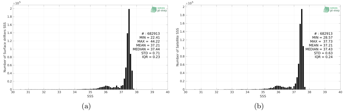
Figure 2: Histograms of SSS from Surface drifters (a) and SMAP SSS L4 OI v2 - Monthly (IPRC) (b) considering all match-up pairs per bins of 0.1 over the Amazon and Orinoco river plumes Pi-MEP region and for the full satellite product period.
