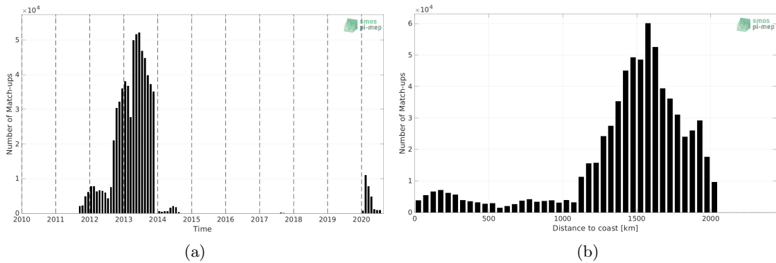
Figure 1: Number of match-ups between Surface drifters and SMAP SSS L4 OI v2 - Monthly (IPRC) SSS as a function of time (a) and as function of the distance to coast (b) over the Amazon and Orinoco river plumes Pi-MEP region and for the full satellite product period.
