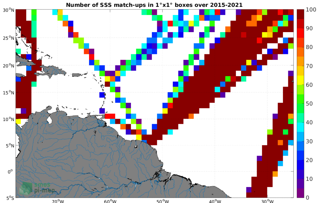
Figure 4: Number of SSS match-ups between TSG (LEGOS-DM) SSS and the SMAP SSS L3 v5 - 8-Day running (RSS) SSS product for the Amazon and Orinoco river plumes Pi-MEP region over 1^\circ \times 1^\circ boxes and for the full satellite product period.
