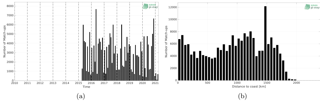
Figure 1: Number of match-ups between TSG (LEGOS-DM) and SMAP SSS L3 v5 - 8-Day running (RSS) SSS as a function of time (a) and as function of the distance to coast (b) over the Amazon and Orinoco river plumes Pi-MEP region and for the full satellite product period.
