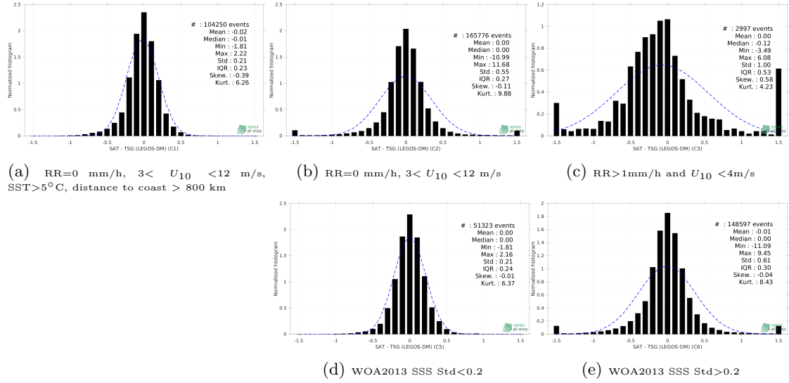
Figure 13: Normalized histogram of \Delta\text{SSS} (SMAP SSS L3 v5 - 8-Day running (RSS) - TSG (LEGOS-DM)) for 5 different subdatasets corresponding to: RR=0 mm/h, 3 < U_{10} < 12 m/s, SST>5°C, distance to coast > 800 km (a), RR=0 mm/h, 3 < U_{10} < 12 m/s (b), RR>1mm/h and U_{10} < 4 m/s (c), WOA2013 SSS Std<0.2 (d), WOA2013 SSS Std>0.2 (e).
