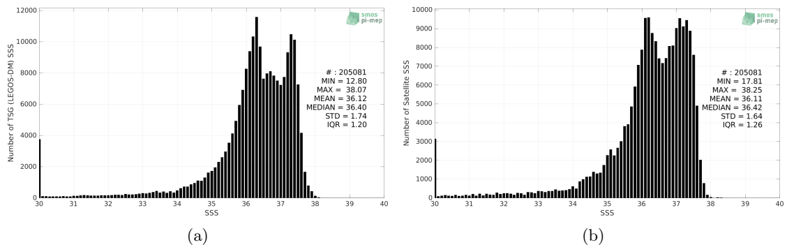
Figure 2: Histograms of SSS from TSG (LEGOS-DM) (a) and SMAP SSS L3 v5 - 8-Day running (RSS) (b) considering all match-up pairs per bins of 0.1 over the Amazon and Orinoco river plumes Pi-MEP region and for the full satellite product period.
