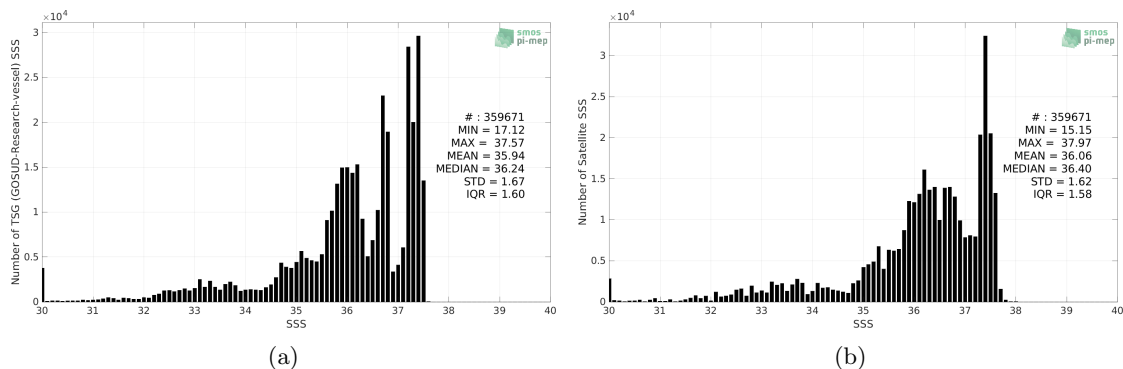
Figure 2: Histograms of SSS from TSG (GOSUD-Research-vessel) (a) and SMAP SSS L3 v5 - 8-Day running (RSS) (b) considering all match-up pairs per bins of 0.1 over the Amazon and Orinoco river plumes Pi-MEP region and for the full satellite product period.
