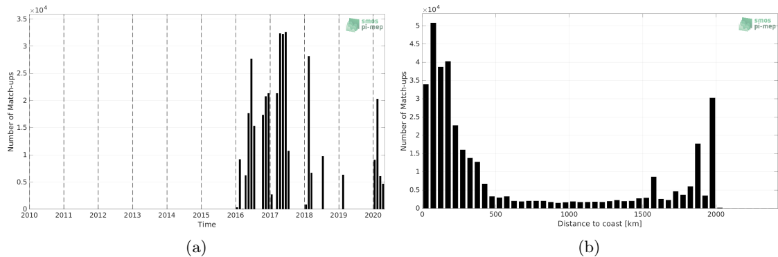
Figure 1: Number of match-ups between TSG (GOSUD-Research-vessel) and SMAP SSS L3 v5 - 8-Day running (RSS) SSS as a function of time (a) and as function of the distance to coast (b) over the Amazon and Orinoco river plumes Pi-MEP region and for the full satellite product period.
