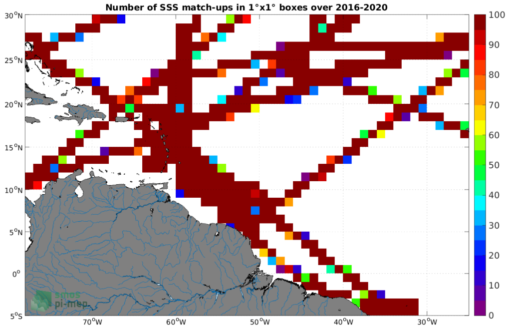
Figure 4: Number of SSS match-ups between TSG (GOSUD-Research-vessel) SSS and the SMAP SSS L3 v5 - 8-Day running (RSS) SSS product for the Amazon and Orinoco river plumes Pi-MEP region over 1^\circ \times 1^\circ boxes and for the full satellite product period.
