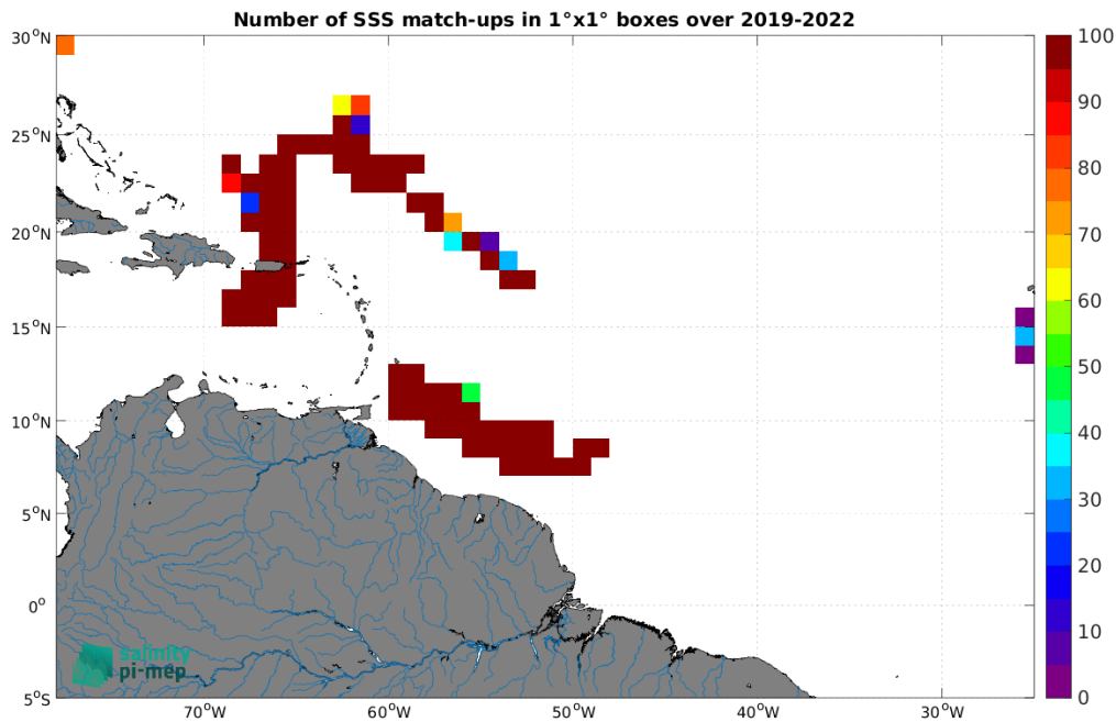
Figure 4: Number of SSS match-ups between Saildrone SSS and the SMAP SSS L3 v5 - 8-Day running (RSS) SSS product for the Amazon and Orinoco river plumes Pi-MEP region over 1^\circ \times 1^\circ boxes and for the full satellite product period.
