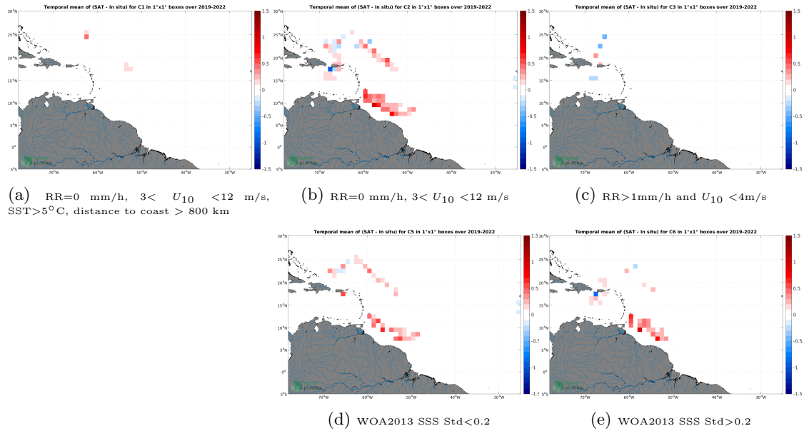
Figure 12: Temporal mean gridded over spatial boxes of size 1^\circ \times 1^\circ of \Delta SSS (SMAP SSS L3 v5 - 8-Day running (RSS) - Saildrone) for 5 different subdatasets corresponding to:RR=0 mm/h, 3 < U_{10} < 12 m/s, SST >5^\circ\text{C} , distance to coast > 800 km (a), RR=0 mm/h, 3 < U_{10} < 12 m/s (b), RR >1 mm/h and U_{10} < 4 m/s (c), WOA2013 SSS Std <0.2 (d), WOA2013 SSS Std >0.2 (e).
