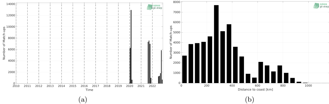
Figure 1: Number of match-ups between Saildrone and SMAP SSS L3 v5 - 8-Day running (RSS) SSS as a function of time (a) and as function of the distance to coast (b) over the Amazon and Orinoco river plumes Pi-MEP region and for the full satellite product period.
