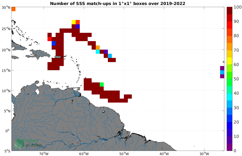
Figure 4: Number of SSS match-ups between Saildrone SSS and the SMAP SSS L3 v5 - 8-Day running (RSS) SSS product for the Amazon and Orinoco river plumes Pi-MEP region over 1^{\circ} \times 1^{\circ} boxes and for the full satellite product period.
