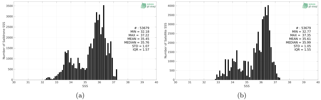
Figure 2: Histograms of SSS from Saildrone (a) and SMAP SSS L3 v5 - 8-Day running (RSS) (b) considering all match-up pairs per bins of 0.1 over the Amazon and Orinoco river plumes Pi-MEP region and for the full satellite product period.
