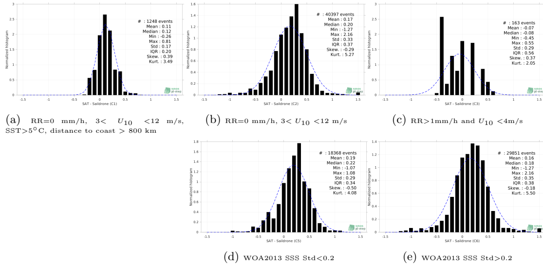
Figure 13: Normalized histogram of \Delta SSS (SMAP SSS L3 v5 - 8-Day running (RSS) - Sairdron) for 5 different subdatasets corresponding to: RR=0 mm/h, 3 < U_{10} < 12 m/s, SST > 5°C, distance to coast > 800 km (a), RR=0 mm/h, 3 < U_{10} < 12 m/s (b), RR > 1mm/h and U_{10} < 4 m/s (c), WOA2013 SSS Std < 0.2 (d), WOA2013 SSS Std > 0.2 (e).
