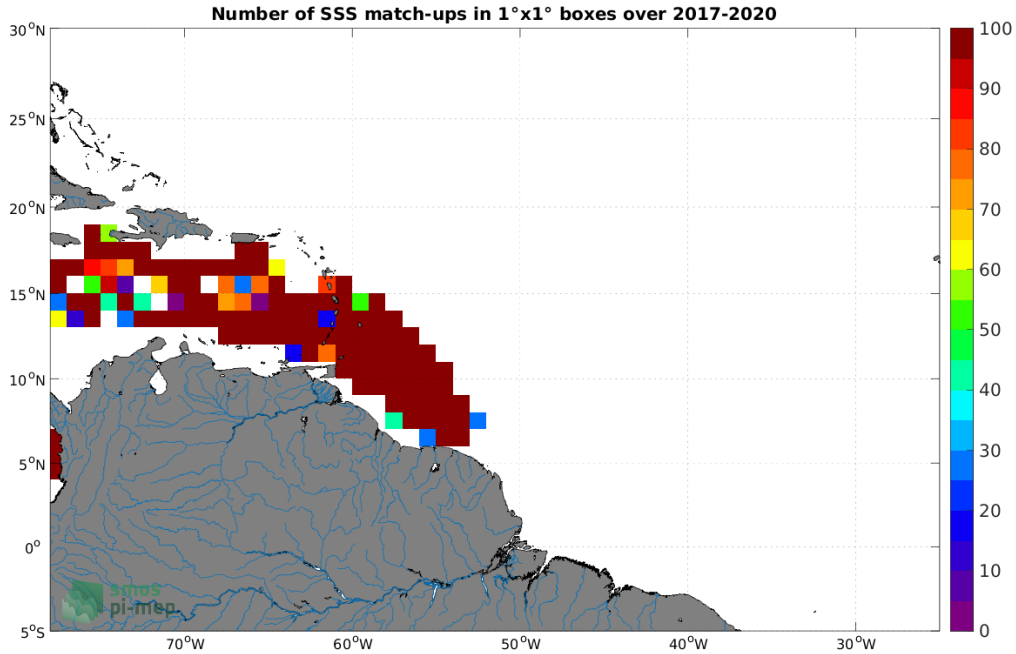
Figure 3: Number of SSS match-ups between Surface drifters SSS and the SMAP SSS L3 v5 - 8-Day running (RSS) SSS product for the Amazon and Orinoco river plumes Pi-MEP region over 1^\circ \times 1^\circ boxes and for the full satellite product period.
