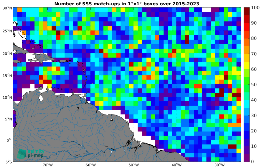
Figure 4: Number of SSS match-ups between Argo SSS and the SMAP SSS L3 v5 - 8-Day running (RSS) SSS product for the Amazon and Orinoco river plumes Pi-MEP region over 1^{\circ} \times 1^{\circ} boxes and for the full satellite product period.
