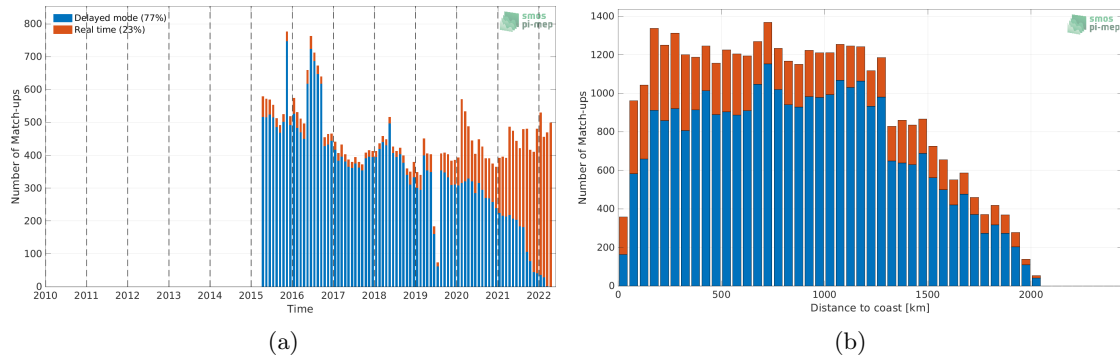
Figure 1: Number of match-ups between Argo and SMAP SSS L3 v5 - 8-Day running (RSS) SSS as a function of time (a) and as function of the distance to coast (b) over the Amazon and Orinoco river plumes Pi-MEP region and for the full satellite product period.
