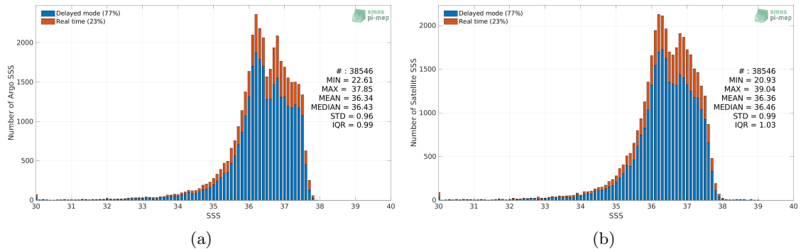
Figure 2: Histograms of SSS from Argo (a) and SMAP SSS L3 v5 - 8-Day running (RSS) (b) considering all match-up pairs per bins of 0.1 over the Amazon and Orinoco river plumes Pi-MEP region and for the full satellite product period.
