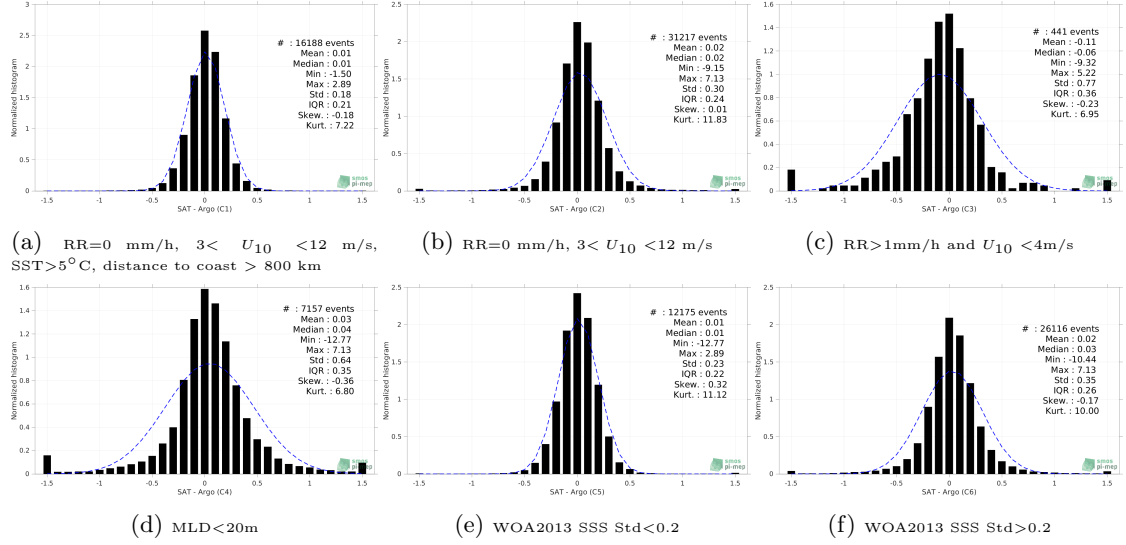
Figure 13: Normalized histogram of \Delta SSS (SMAP SSS L3 v5 - 8-Day running (RSS) - Argo) for 6 different subdatasets corresponding to: RR=0 mm/h, 3 < U_{10} < 12 m/s, SST > 5°C, distance to coast > 800 km (a), RR=0 mm/h, 3 < U_{10} < 12 m/s (b), RR > 1mm/h and U_{10} < 4 m/s (c), MLD < 20m (d), WOA2013 SSS Std < 0.2 (e), WOA2013 SSS Std > 0.2 (f).
