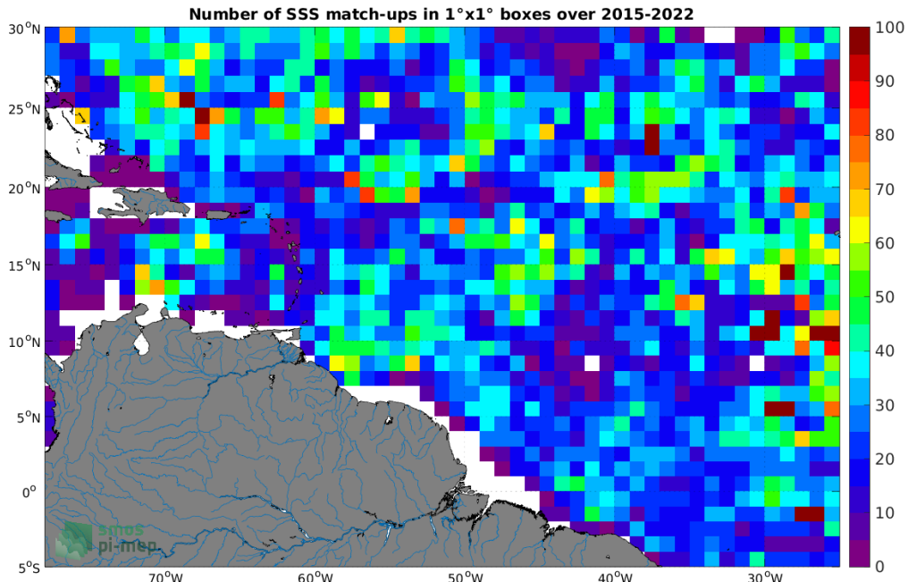
Figure 4: Number of SSS match-ups between Argo SSS and the SMAP SSS L3 v5 - 8-Day running (RSS) SSS product for the Amazon and Orinoco river plumes Pi-MEP region over 1^\circ \times 1^\circ boxes and for the full satellite product period.
