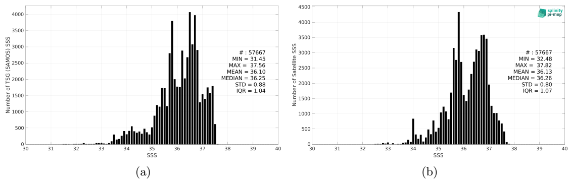
Figure 2: Histograms of SSS from TSG (SAMOS) (a) and SMAP SSS L3 v5 - Monthly (RSS) (b) considering all match-up pairs per bins of 0.1 over the Amazon and Orinoco river plumes Pi-MEP region and for the full satellite product period.
