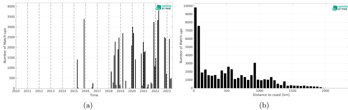
Figure 1: Number of match-ups between TSG (SAMOS) and SMAP SSS L3 v5 - Monthly (RSS) SSS as a function of time (a) and as function of the distance to coast (b) over the Amazon and Orinoco river plumes Pi-MEP region and for the full satellite product period.
