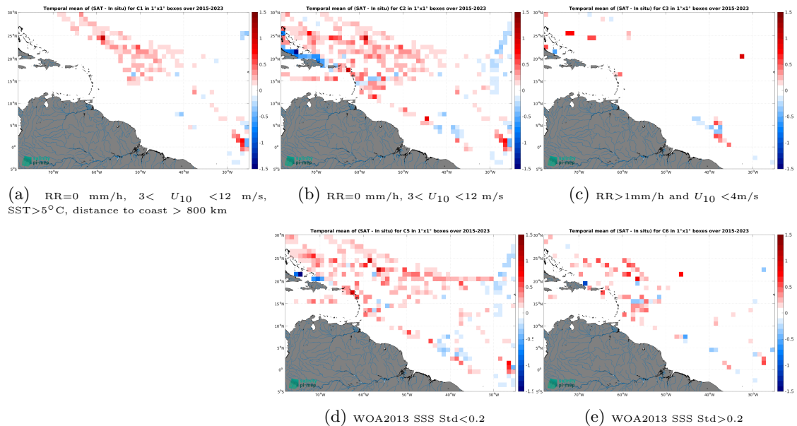
Figure 12: Temporal mean gridded over spatial boxes of size 1^\circ \times 1^\circ of \Delta\text{SSS} (SMAP SSS L3 v5 - Monthly (RSS) - TSG (SAMOS)) for 5 different subdatasets corresponding to:RR=0 mm/h, 3 < U_{10} < 12 m/s, SST >5^\circ\text{C} , distance to coast > 800 km (a), RR=0 mm/h, 3 < U_{10} < 12 m/s (b), RR >1 mm/h and U_{10} < 4 m/s (c), WOA2013 SSS Std <0.2 (d), WOA2013 SSS Std >0.2 (e).
