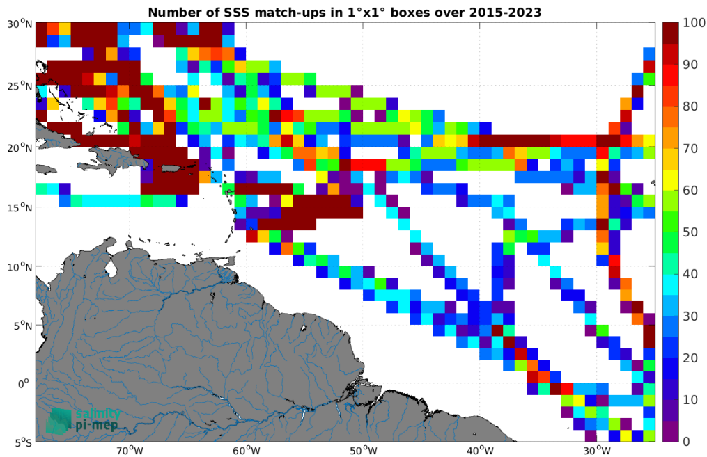
Figure 4: Number of SSS match-ups between TSG (SAMOS) SSS and the SMAP SSS L3 v5 - Monthly (RSS) SSS product for the Amazon and Orinoco river plumes Pi-MEP region over 1^\circ \times 1^\circ boxes and for the full satellite product period.
