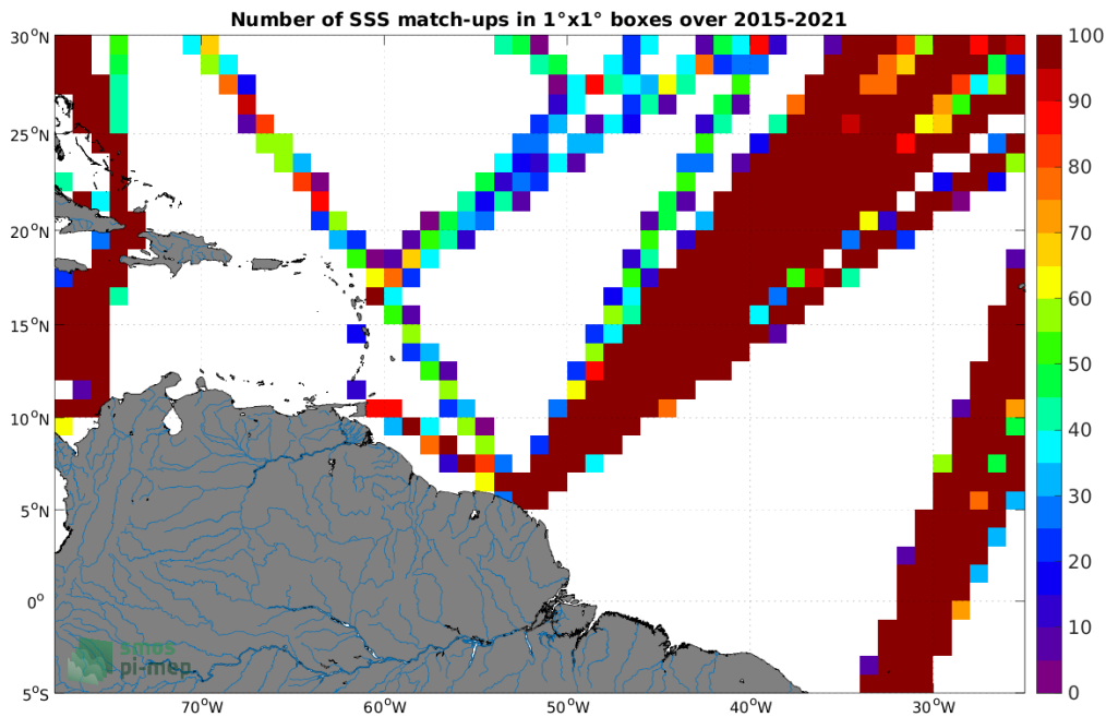
Figure 4: Number of SSS match-ups between TSG (LEGOS-DM) SSS and the SMAP SSS L3 v5 - Monthly (RSS) SSS product for the Amazon and Orinoco river plumes Pi-MEP region over 1^\circ \times 1^\circ boxes and for the full satellite product period.
