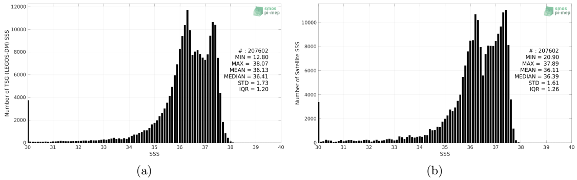
Figure 2: Histograms of SSS from TSG (LEGOS-DM) (a) and SMAP SSS L3 v5 - Monthly (RSS) (b) considering all match-up pairs per bins of 0.1 over the Amazon and Orinoco river plumes Pi-MEP region and for the full satellite product period.
