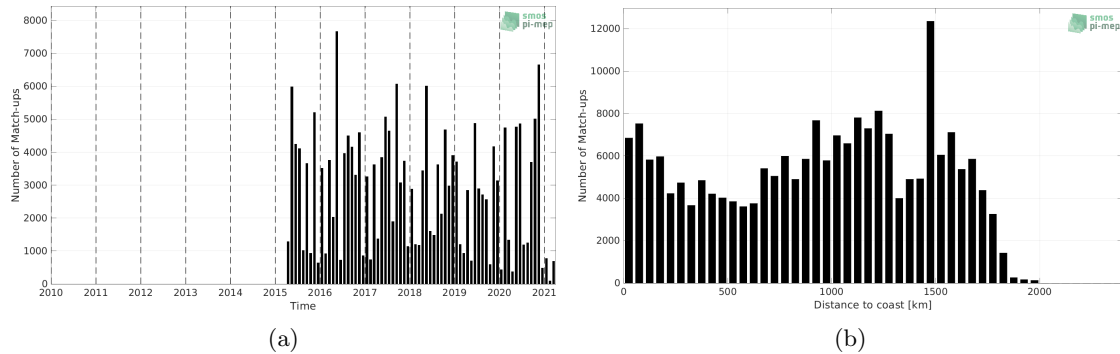
Figure 1: Number of match-ups between TSG (LEGOS-DM) and SMAP SSS L3 v5 - Monthly (RSS) SSS as a function of time (a) and as function of the distance to coast (b) over the Amazon and Orinoco river plumes Pi-MEP region and for the full satellite product period.
