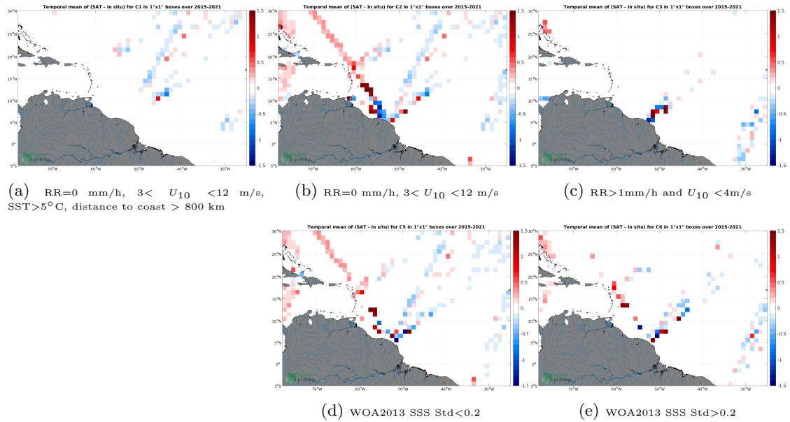
Figure 12: Temporal mean gridded over spatial boxes of size 1^\circ \times 1^\circ of \Delta SSS (SMAP SSS L3 v5 - Monthly (RSS) - TSG (LEGOS-DM)) for 5 different subdatasets corresponding to:RR=0 mm/h, 3 < U_{10} < 12 m/s, SST >5^\circ C, distance to coast > 800 km (a), RR=0 mm/h, 3 < U_{10} < 12 m/s (b), RR >1 mm/h and U_{10} < 4 m/s (c), WOA2013 SSS Std <0.2 (d), WOA2013 SSS Std >0.2 (e).
