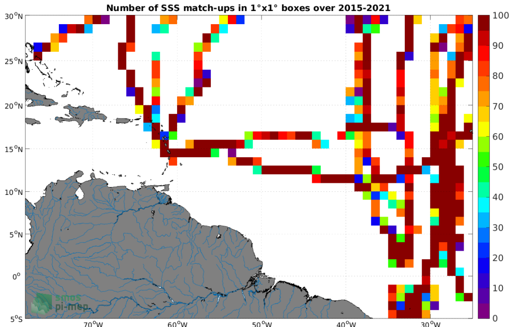
Figure 4: Number of SSS match-ups between TSG (GOSUD-Sailing-ship) SSS and the SMAP SSS L3 v5 - Monthly (RSS) SSS product for the Amazon and Orinoco river plumes Pi-MEP region over 1^\circ \times 1^\circ boxes and for the full satellite product period.
