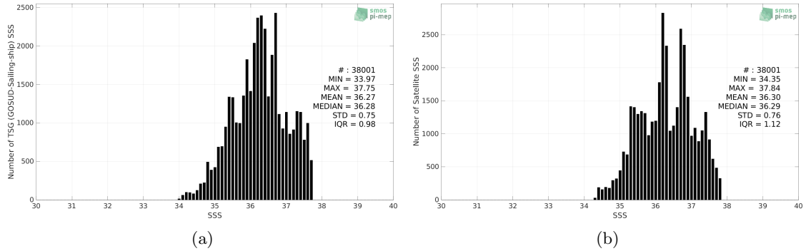
Figure 2: Histograms of SSS from TSG (GOSUD-Sailing-ship) (a) and SMAP SSS L3 v5 - Monthly (RSS) (b) considering all match-up pairs per bins of 0.1 over the Amazon and Orinoco river plumes Pi-MEP region and for the full satellite product period.
