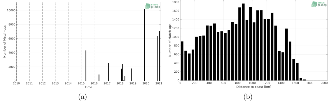
Figure 1: Number of match-ups between TSG (GOSUD-Sailing-ship) and SMAP SSS L3 v5 - Monthly (RSS) SSS as a function of time (a) and as function of the distance to coast (b) over the Amazon and Orinoco river plumes Pi-MEP region and for the full satellite product period.
