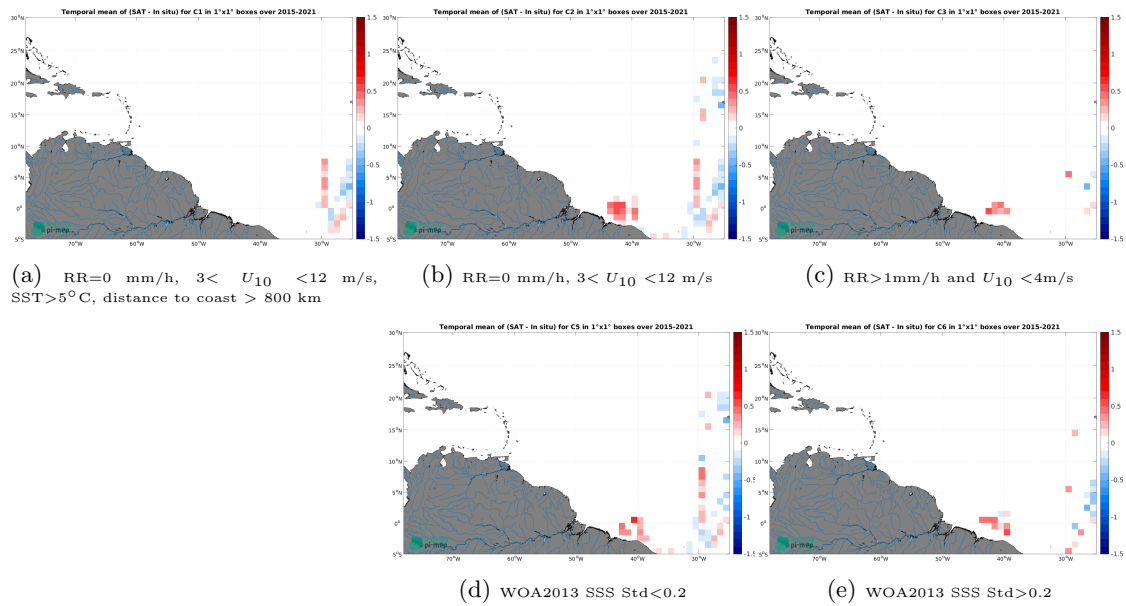
Figure 12: Temporal mean gridded over spatial boxes of size 1^\circ \times 1^\circ of \Delta SSS (SMAP SSS L3 v5 - Monthly (RSS) - TSG (CSIC-UTM)) for 5 different subdatasets corresponding to:RR=0 mm/h, 3 < U_{10} < 12 m/s, SST >5^\circ\text{C} , distance to coast > 800 km (a), RR=0 mm/h, 3 < U_{10} < 12 m/s (b), RR >1 mm/h and U_{10} < 4 m/s (c), WOA2013 SSS Std <0.2 (d), WOA2013 SSS Std >0.2 (e).
