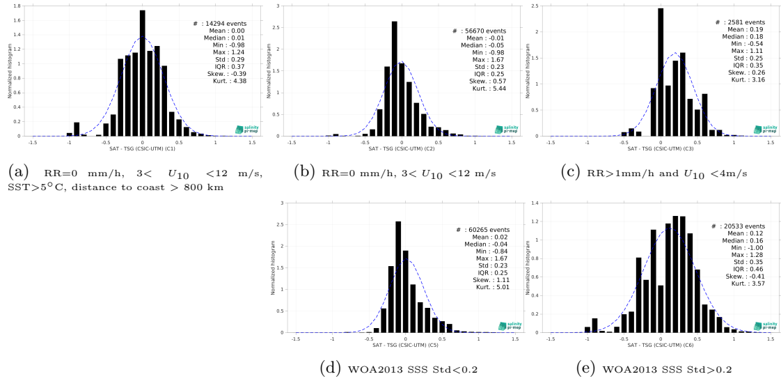
Figure 13: Normalized histogram of \Delta SSS (SMAP SSS L3 v5 - Monthly (RSS) - TSG (CSIC-UTM)) for 5 different subdatasets corresponding to: RR=0 mm/h, 3 < U_{10} < 12 m/s, SST>5°C, distance to coast > 800 km (a), RR=0 mm/h, 3 < U_{10} < 12 m/s (b), RR>1mm/h and U_{10} < 4 m/s (c), WOA2013 SSS Std<0.2 (d), WOA2013 SSS Std>0.2 (e).
