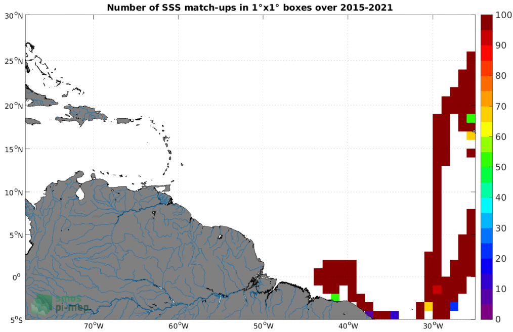
Figure 4: Number of SSS match-ups between TSG (CSIC-UTM) SSS and the SMAP SSS L3 v5 - Monthly (RSS) SSS product for the Amazon and Orinoco river plumes Pi-MEP region over 1^\circ \times 1^\circ boxes and for the full satellite product period.
