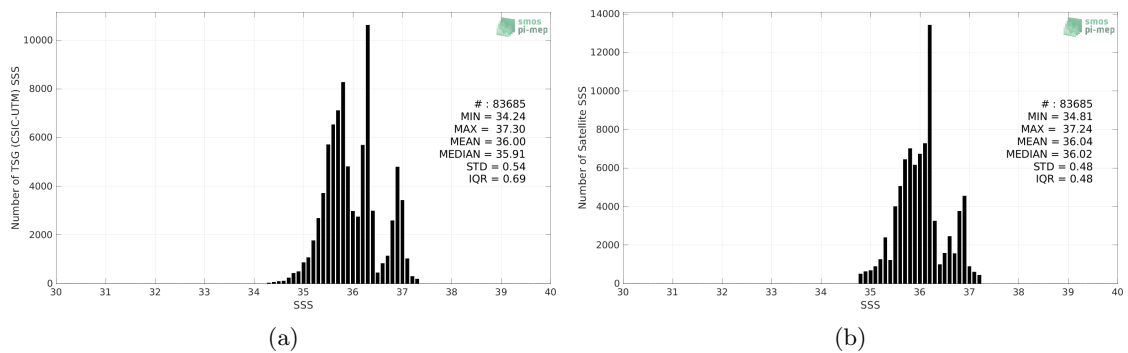
Figure 2: Histograms of SSS from TSG (CSIC-UTM) (a) and SMAP SSS L3 v5 - Monthly (RSS) (b) considering all match-up pairs per bins of 0.1 over the Amazon and Orinoco river plumes Pi-MEP region and for the full satellite product period.
