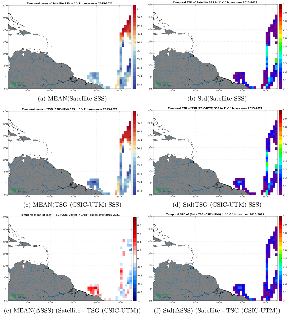
Figure 6: Temporal mean (left) and Std (right) of SSS from SMAP SSS L3 v5 - Monthly (RSS) (top), TSG (CSIC-UTM) (middle), and of \Delta SSS (Satellite - TSG (CSIC-UTM)). Only match-up pairs are used to generate these maps.
