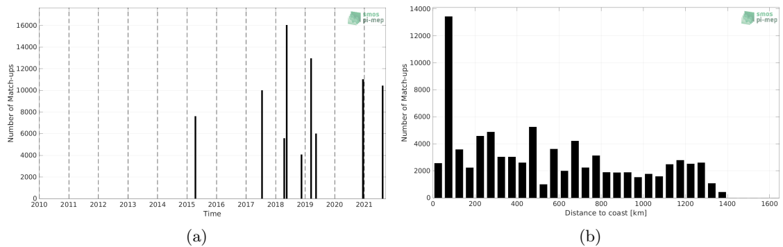
Figure 1: Number of match-ups between TSG (CSIC-UTM) and SMAP SSS L3 v5 - Monthly (RSS) SSS as a function of time (a) and as function of the distance to coast (b) over the Amazon and Orinoco river plumes Pi-MEP region and for the full satellite product period.
