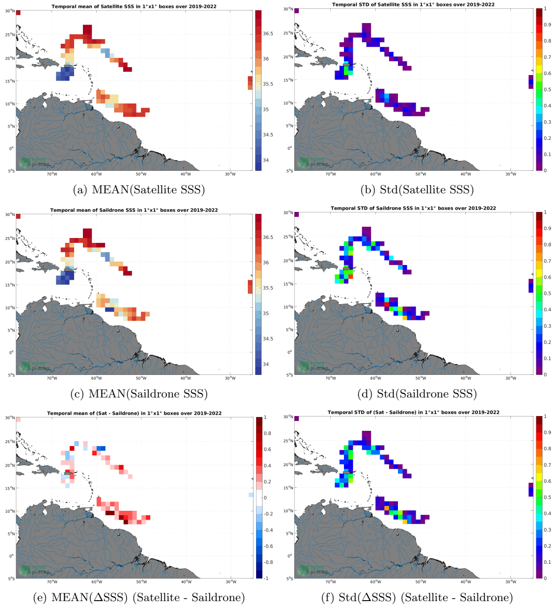
Figure 6: Temporal mean (left) and Std (right) of SSS from SMAP SSS L3 v5 - Monthly (RSS) (top), Saildrone (middle), and of \Delta SSS (Satellite - Saildrone). Only match-up pairs are used to generate these maps.
