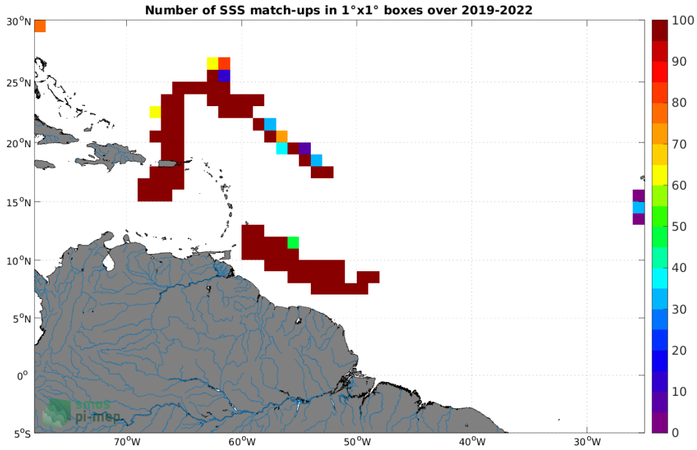
Figure 4: Number of SSS match-ups between Saildrone SSS and the SMAP SSS L3 v5 - Monthly (RSS) SSS product for the Amazon and Orinoco river plumes Pi-MEP region over 1°x1° boxes and for the full satellite product period.
