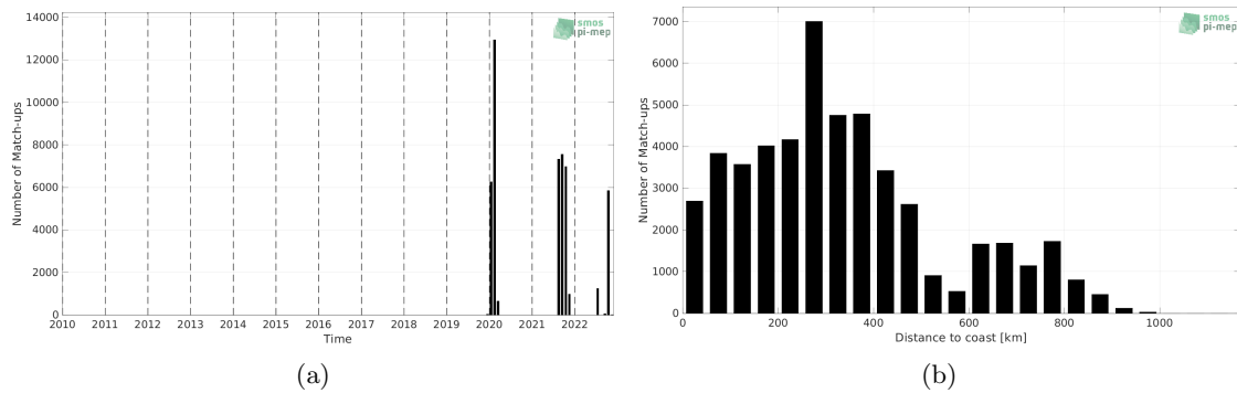
Figure 1: Number of match-ups between Saildrone and SMAP SSS L3 v5 - Monthly (RSS) SSS as a function of time (a) and as function of the distance to coast (b) over the Amazon and Orinoco river plumes Pi-MEP region and for the full satellite product period.
