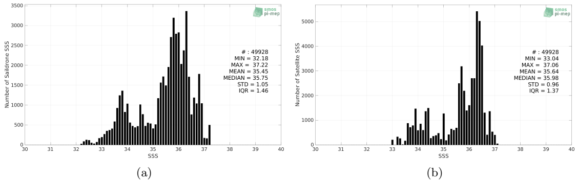
Figure 2: Histograms of SSS from Saïdrone (a) and SMAP SSS L3 v5 - Monthly (RSS) (b) considering all match-up pairs per bins of 0.1 over the Amazon and Orinoco river plumes Pi-MEP region and for the full satellite product period.
