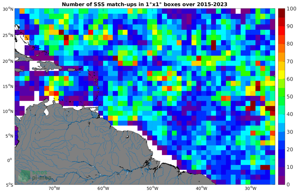
Figure 4: Number of SSS match-ups between Argo SSS and the SMAP SSS L3 v5 - Monthly (RSS) SSS product for the Amazon and Orinoco river plumes Pi-MEP region over 1^{\circ} \times 1^{\circ} boxes and for the full satellite product period.
