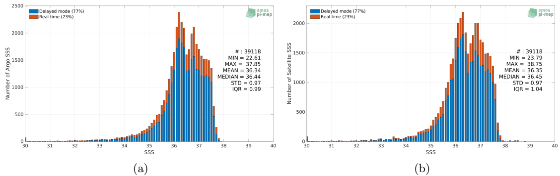
Figure 2: Histograms of SSS from Argo (a) and SMAP SSS L3 v5 - Monthly (RSS) (b) considering all match-up pairs per bins of 0.1 over the Amazon and Orinoco river plumes Pi-MEP region and for the full satellite product period.
