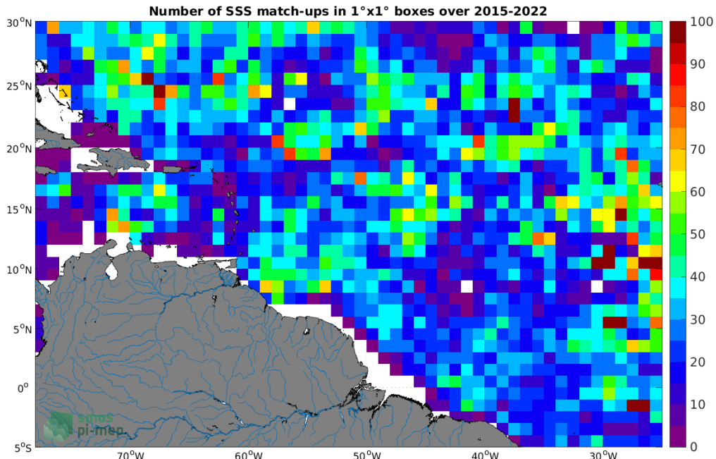
Figure 4: Number of SSS match-ups between Argo SSS and the SMAP SSS L3 v5 - Monthly (RSS) SSS product for the Amazon and Orinoco river plumes Pi-MEP region over 1^\circ \times 1^\circ boxes and for the full satellite product period.
