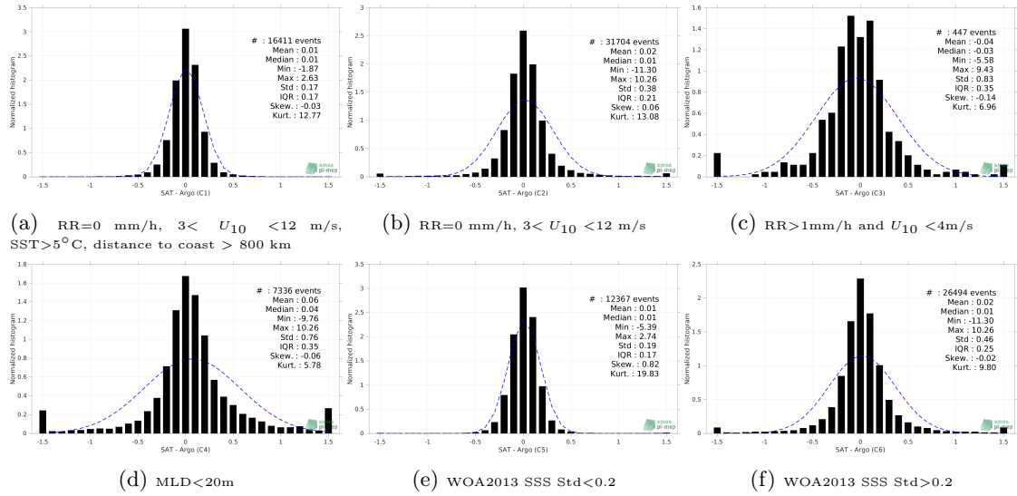
Figure 13: Normalized histogram of \Delta SSS (SMAP SSS L3 v5 - Monthly (RSS) - Argo) for 6 different subdatasets corresponding to: RR=0 mm/h, 3 < U_{10} < 12 m/s, SST > 5°C, distance to coast > 800 km (a), RR=0 mm/h, 3 < U_{10} < 12 m/s (b), RR > 1mm/h and U_{10} < 4 m/s (c), MLD < 20m (d), WOA2013 SSS Std < 0.2 (e), WOA2013 SSS Std > 0.2 (f).
