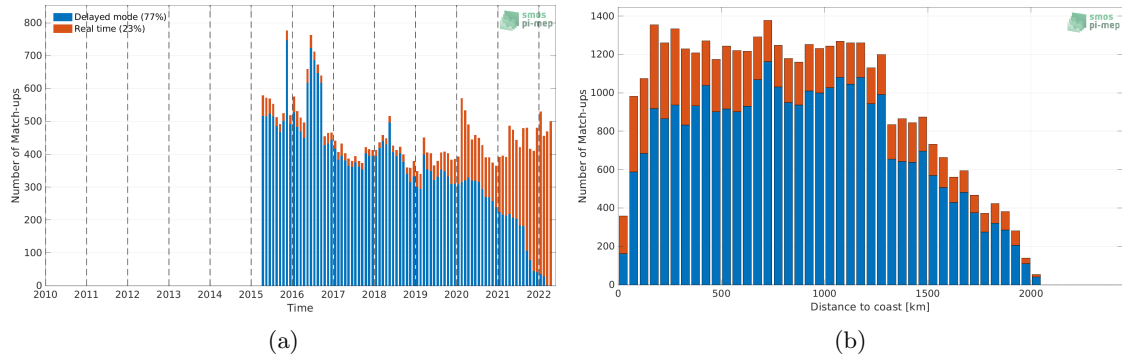
Figure 1: Number of match-ups between Argo and SMAP SSS L3 v5 - Monthly (RSS) SSS as a function of time (a) and as function of the distance to coast (b) over the Amazon and Orinoco river plumes Pi-MEP region and for the full satellite product period.
