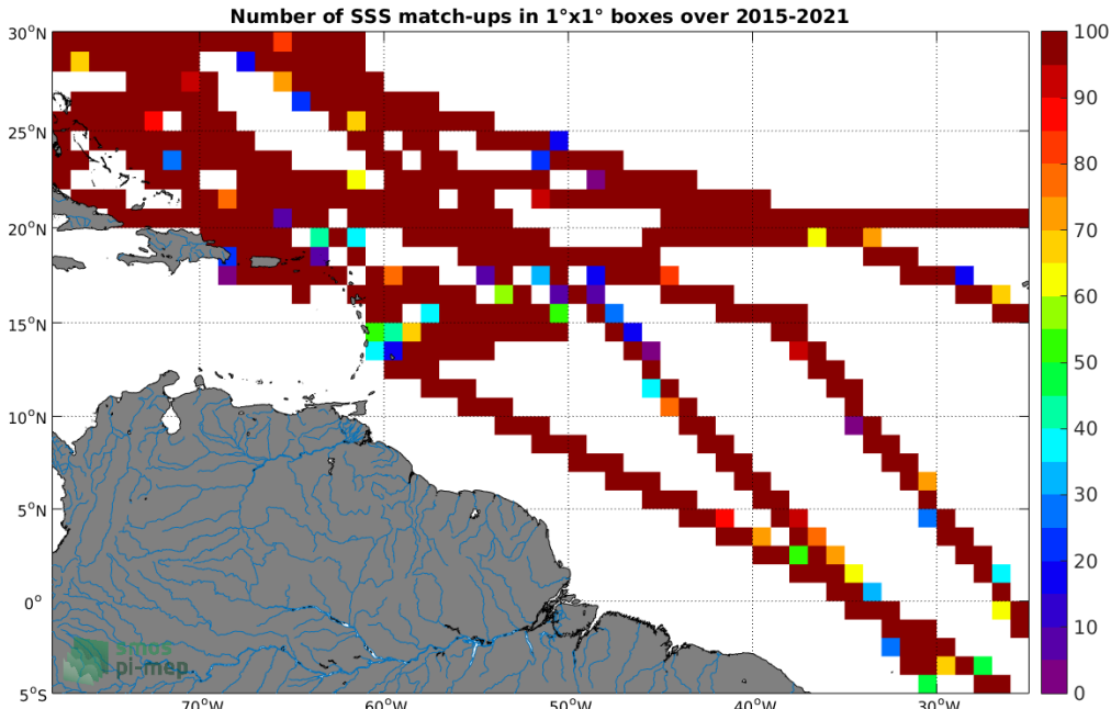
Figure 4: Number of SSS match-ups between TSG (SAMOS) SSS and the SMAP SSS L3 v4 - 8-Day running (RSS) SSS product for the Amazon and Orinoco river plumes Pi-MEP region over 1^{\circ} \times 1^{\circ} boxes and for the full satellite product period.
