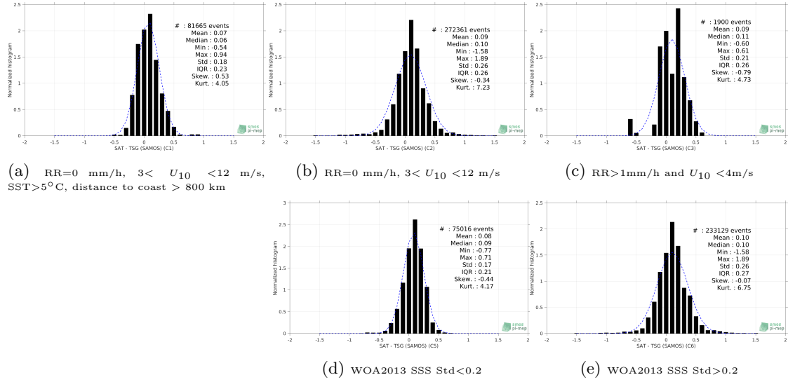
Figure 13: Normalized histogram of \Delta SSS (SMAP SSS L3 v4 - 8-Day running (RSS) - TSG (SAMOS)) for 5 different subdatasets corresponding to: RR=0 mm/h, 3 < U_{10} < 12 m/s, SST > 5^\circ C , distance to coast > 800 km (a), RR=0 mm/h, 3 < U_{10} < 12 m/s (b), RR > 1 mm/h and U_{10} < 4 m/s (c), WOA2013 SSS Std < 0.2 (d), WOA2013 SSS Std > 0.2 (e).
