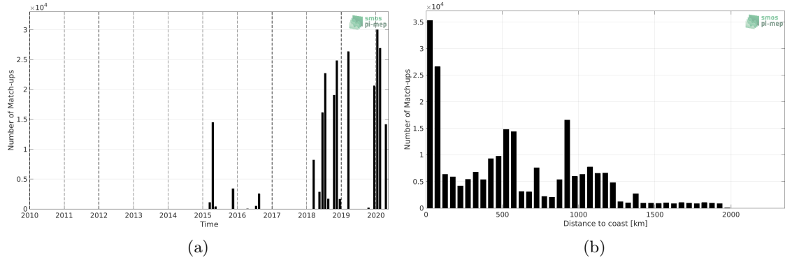
Figure 1: Number of match-ups between TSG (SAMOS) and SMAP SSS L3 v4 - 8-Day running (RSS) SSS as a function of time (a) and as function of the distance to coast (b) over the Amazon and Orinoco river plumes Pi-MEP region and for the full satellite product period.
