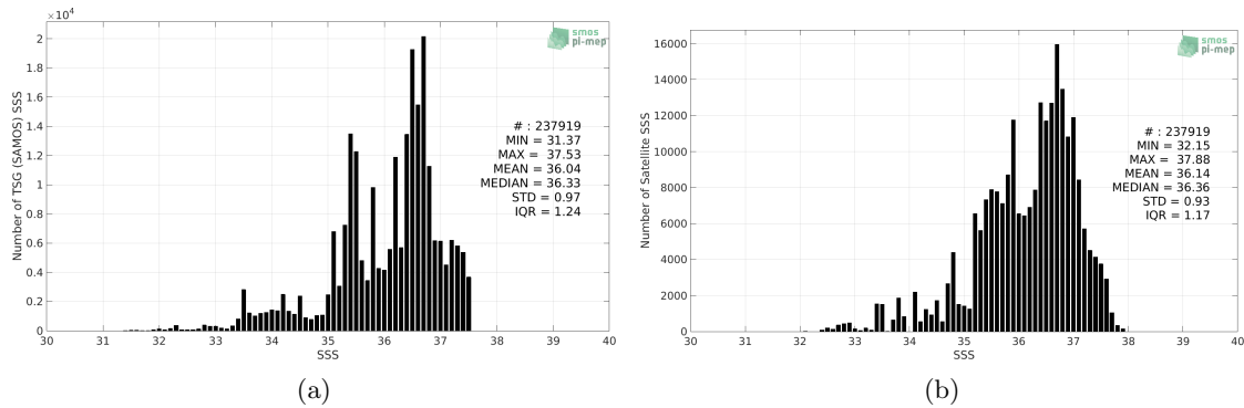
Figure 2: Histograms of SSS from TSG (SAMOS) (a) and SMAP SSS L3 v4 - 8-Day running (RSS) (b) considering all match-up pairs per bins of 0.1 over the Amazon and Orinoco river plumes Pi-MEP region and for the full satellite product period.
