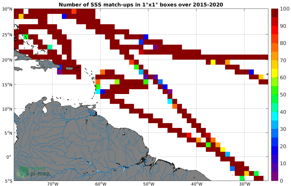
Figure 4: Number of SSS match-ups between TSG (SAMOS) SSS and the SMAP SSS L3 v4 - 8-Day running (RSS) SSS product for the Amazon and Orinoco river plumes Pi-MEP region over 1°x1° boxes and for the full satellite product period.
