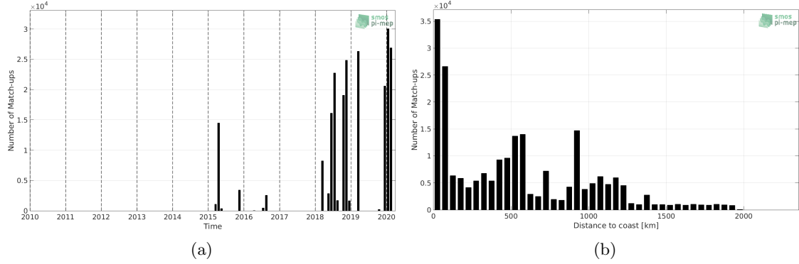
Figure 1: Number of match-ups between TSG-SAMOS and SMAP-L3-RSS-V4-8DAY-RUNNING SSS as a function of time (a) and as function of the distance to coast (b) over the Amazon and Orinoco river plumes Pi-MEP region and for the full satellite product period.
