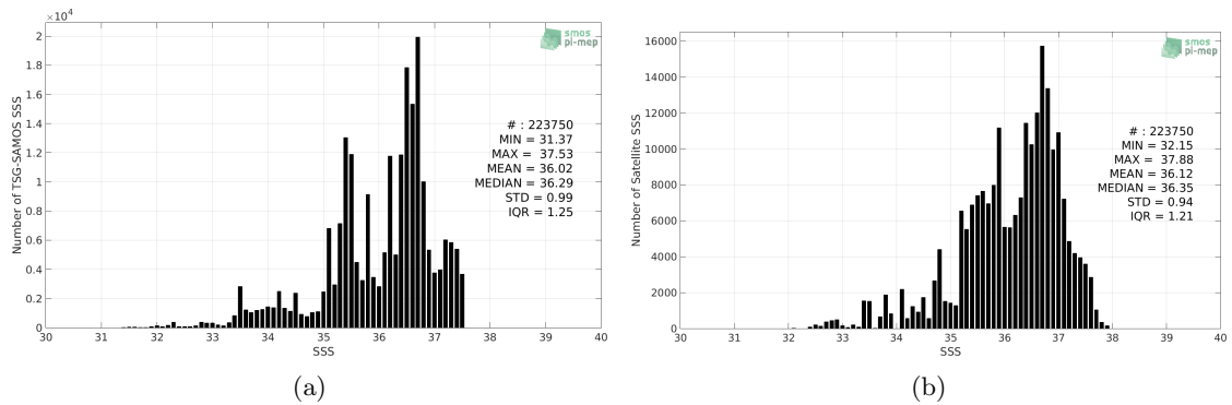
Figure 2: Histograms of SSS from TSG-SAMOS (a) and SMAP-L3-RSS-V4-8DAY-RUNNING (b) considering all match-up pairs per bins of 0.1 over the Amazon and Orinoco river plumes Pi-MEP region and for the full satellite product period.
