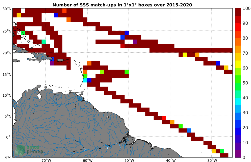
Figure 4: Number of SSS match-ups between TSG-SAMOS SSS and the SMAP-L3-RSS-V4-8DAY-RUNNING SSS product for the Amazon and Orinoco river plumes Pi-MEP region over 1^\circ \times 1^\circ boxes and for the full satellite product period.
