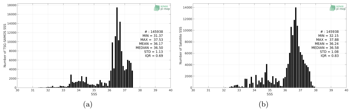
Figure 2: Histograms of SSS from TSG-SAMOS (a) and SMAP-L3-RSS-V4-8DAY-RUNNING (b) considering all match-up pairs per bins of 0.1 over the Amazon and Orinoco river plumes Pi-MEP region and for the full satellite product period.
