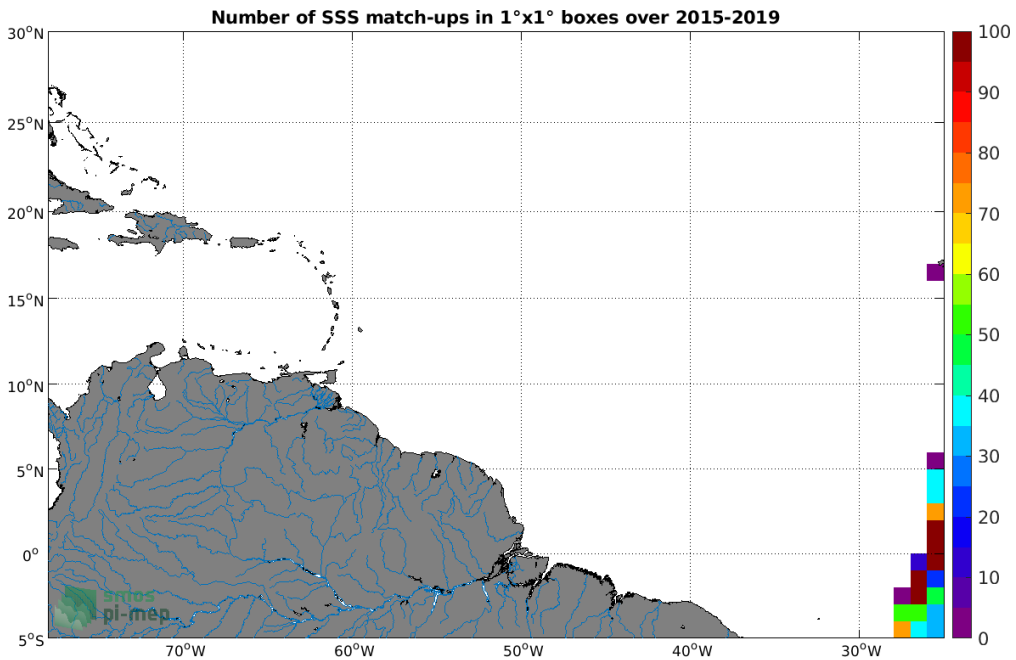
Figure 4: Number of SSS match-ups between TSG (Polarstern) SSS and the SMAP SSS L3 v4 - 8-Day running (RSS) SSS product for the Amazon and Orinoco river plumes Pi-MEP region over 1°x1° boxes and for the full satellite product period.
