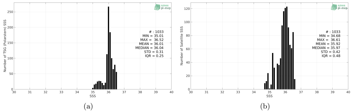
Figure 2: Histograms of SSS from TSG (Polarstern) (a) and SMAP SSS L3 v4 - 8-Day running (RSS) (b) considering all match-up pairs per bins of 0.1 over the Amazon and Orinoco river plumes Pi-MEP region and for the full satellite product period.
