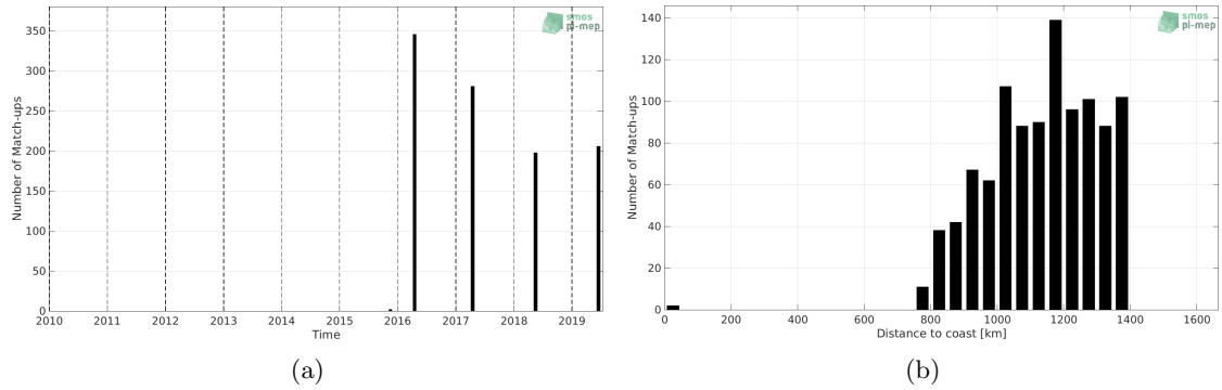
Figure 1: Number of match-ups between TSG (Polarstern) and SMAP SSS L3 v4 - 8-Day running (RSS) SSS as a function of time (a) and as function of the distance to coast (b) over the Amazon and Orinoco river plumes Pi-MEP region and for the full satellite product period.
