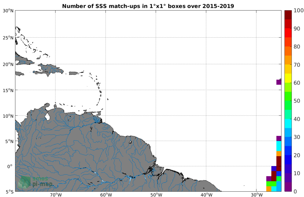
Figure 4: Number of SSS match-ups between TSG (Polarstern) SSS and the SMAP SSS L3 v4 - 8-Day running (RSS) SSS product for the Amazon and Orinoco river plumes Pi-MEP region over 1^\circ \times 1^\circ boxes and for the full satellite product period.
