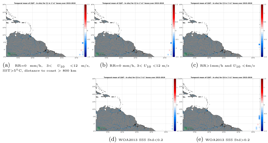
Figure 12: Temporal mean gridded over spatial boxes of size 1°x1° of \Delta SSS (SMAP SSS L3 v4 - 8-Day running (RSS) - TSG (Polarstern)) for 5 different subdatasets corresponding to:RR=0 mm/h, 3 < U_{10} < 12 m/s, SST>5°C, distance to coast > 800 km (a), RR=0 mm/h, 3 < U_{10} < 12 m/s (b), RR>1mm/h and U_{10} < 4 m/s (c), WOA2013 SSS Std<0.2 (d), WOA2013 SSS Std>0.2 (e).
