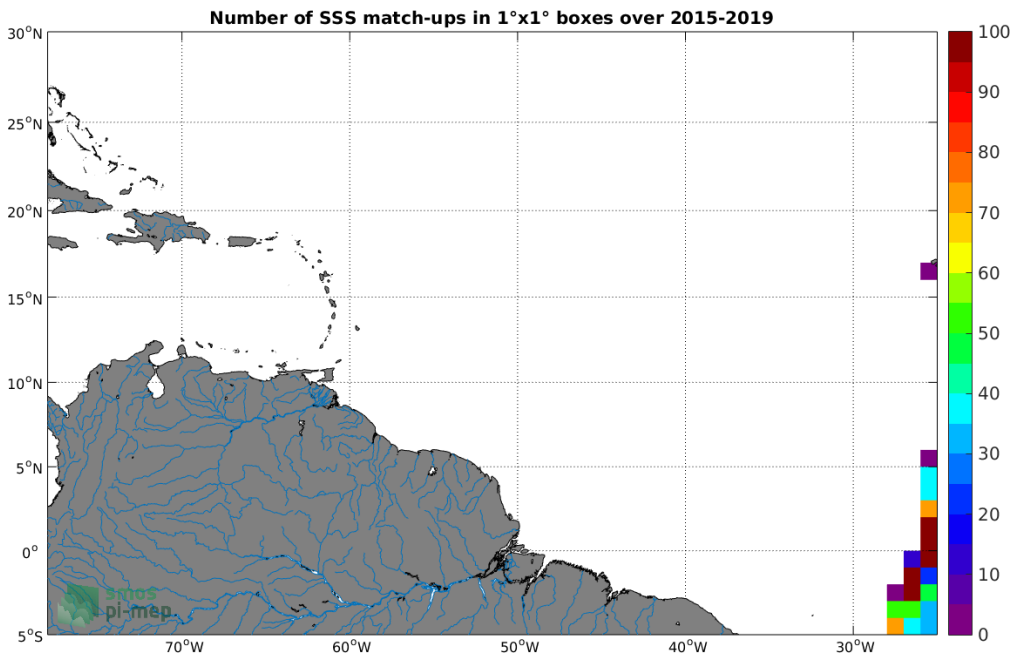
Figure 4: Number of SSS match-ups between TSG-POLARSTERN SSS and the SMAP-L3-RSS-V4-8DAY-RUNNING SSS product for the Amazon and Orinoco river plumes Pi-MEP region over 1^\circ \times 1^\circ boxes and for the full satellite product period.
