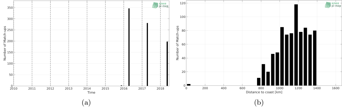
Figure 1: Number of match-ups between TSG-POLARSTERN and SMAP-L3-RSS-V4-8DAY-RUNNING SSS as a function of time (a) and as function of the distance to coast (b) over the Amazon and Orinoco river plumes Pi-MEP region and for the full satellite product period.
