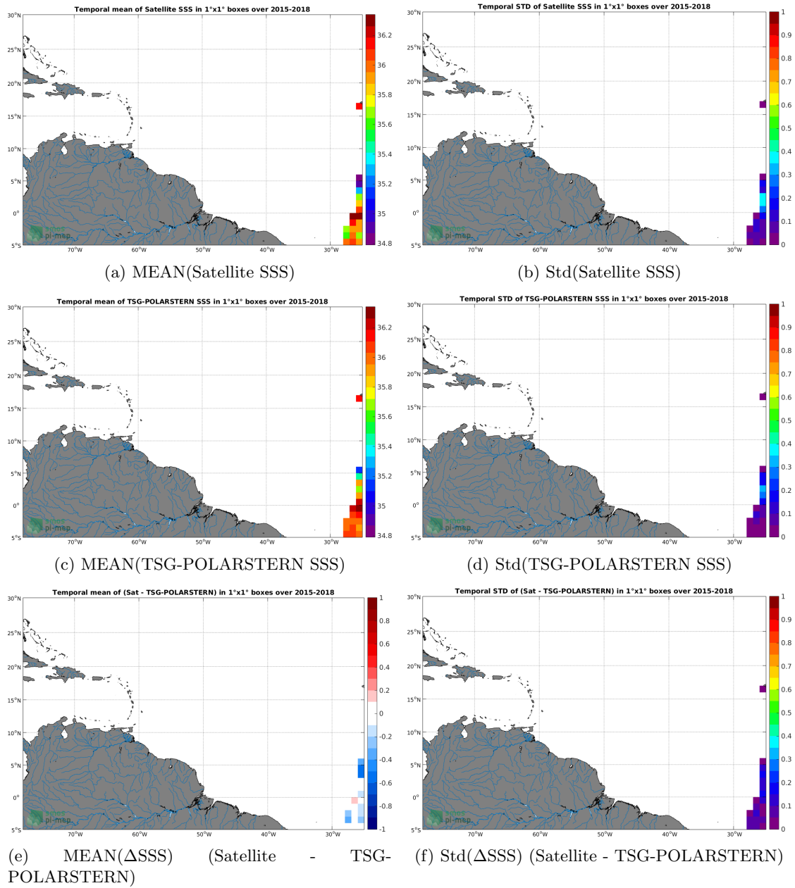
Figure 6: Temporal mean (left) and Std (right) of SSS from SMAP-L3-RSS-V4-8DAY-RUNNING (top), TSG-POLARSTERN (middle), and of \Delta SSS (Satellite - TSG-POLARSTERN). Only match-up pairs are used to generate these maps.
