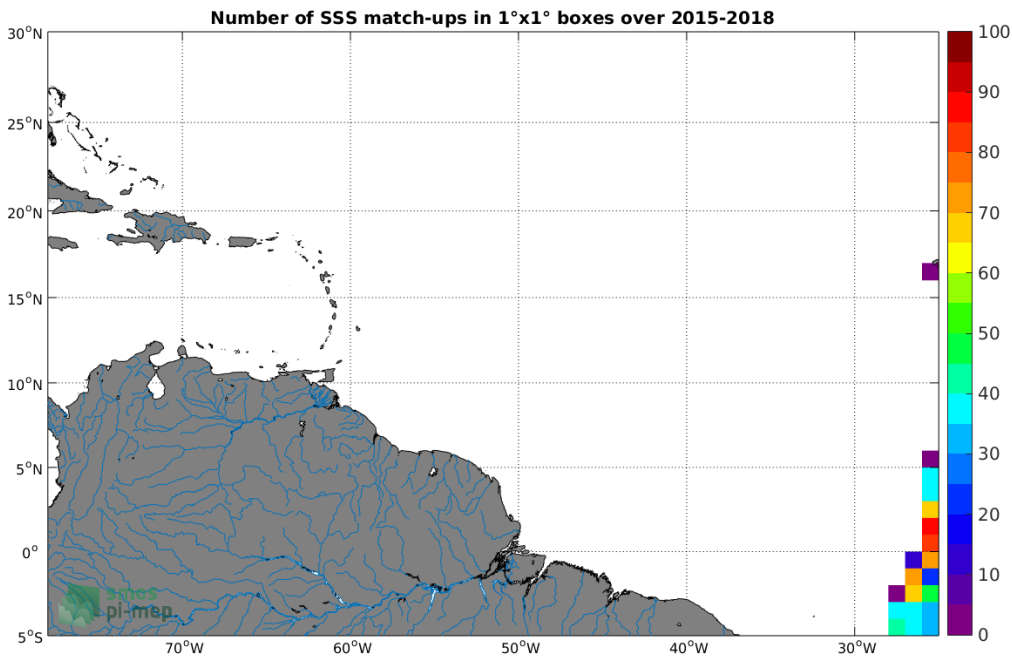
Figure 4: Number of SSS match-ups between TSG-POLARSTERN SSS and the SMAP-L3-RSS-V4-8DAY-RUNNING SSS product for the Amazon and Orinoco river plumes Pi-MEP region over 1°x1° boxes and for the full satellite product period.
