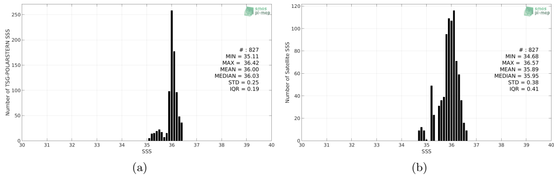
Figure 2: Histograms of SSS from TSG-POLARSTERN (a) and SMAP-L3-RSS-V4-8DAY-RUNNING (b) considering all match-up pairs per bins of 0.1 over the Amazon and Orinoco river plumes Pi-MEP region and for the full satellite product period.
