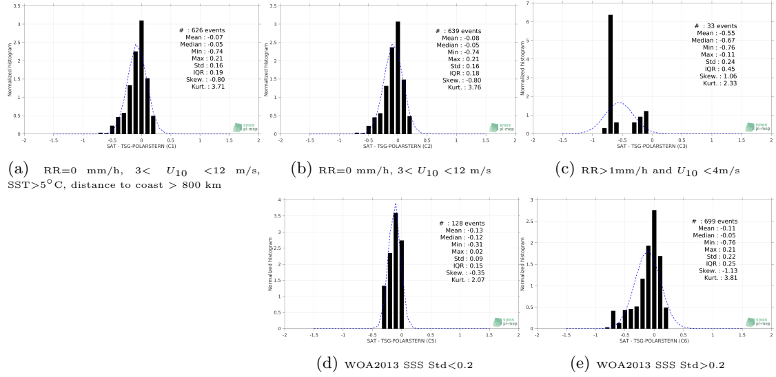
Figure 13: Normalized histogram of \Delta SSS (SMAP-L3-RSS-V4-8DAY-RUNNING - TSG-POLARSTERN) for 5 different subdatasets corresponding to: RR=0 mm/h, 3 < U_{10} < 12 m/s, SST>5°C, distance to coast > 800 km (a), RR=0 mm/h, 3 < U_{10} < 12 m/s (b), RR>1mm/h and U_{10} < 4 m/s (c), WOA2013 SSS Std<0.2 (d), WOA2013 SSS Std>0.2 (e).
