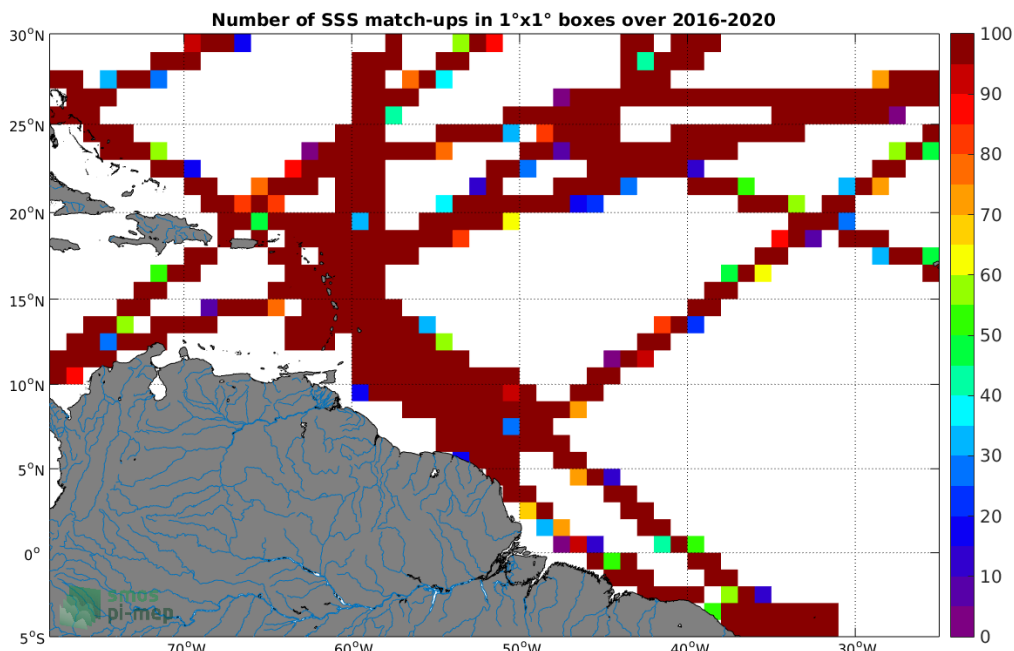
Figure 4: Number of SSS match-ups between TSG (GOSUD-Research-vessel) SSS and the SMAP SSS L3 v4 - 8-Day running (RSS) SSS product for the Amazon and Orinoco river plumes Pi-MEP region over 1^{\circ} \times 1^{\circ} boxes and for the full satellite product period.
