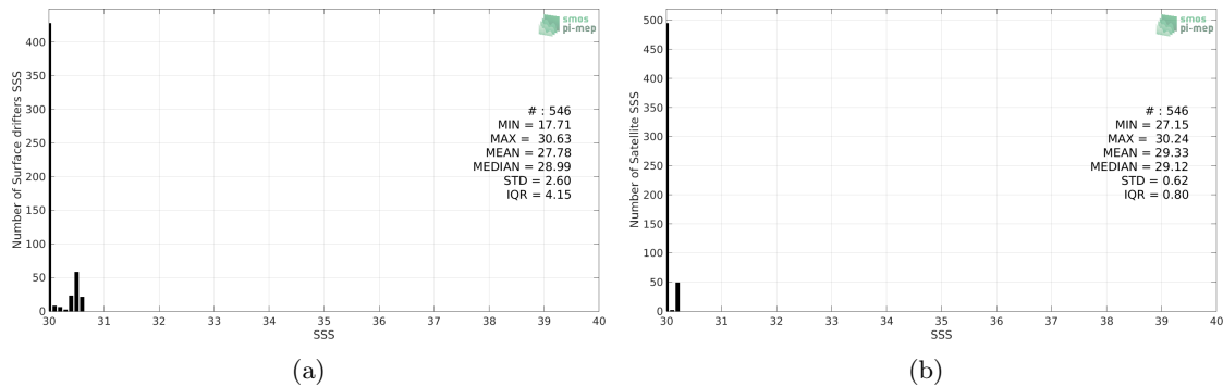
Figure 2: Histograms of SSS from Surface drifters (a) and SMAP SSS L3 v4 - 8-Day running (RSS) (b) considering all match-up pairs per bins of 0.1 over the Amazon and Orinoco river plumes Pi-MEP region and for the full satellite product period.
