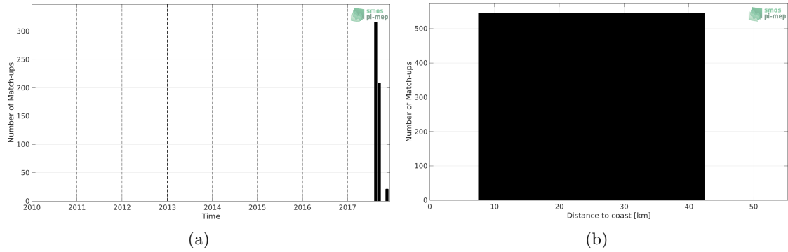
Figure 1: Number of match-ups between Surface drifters and SMAP SSS L3 v4 - 8-Day running (RSS) SSS as a function of time (a) and as function of the distance to coast (b) over the Amazon and Orinoco river plumes Pi-MEP region and for the full satellite product period.
