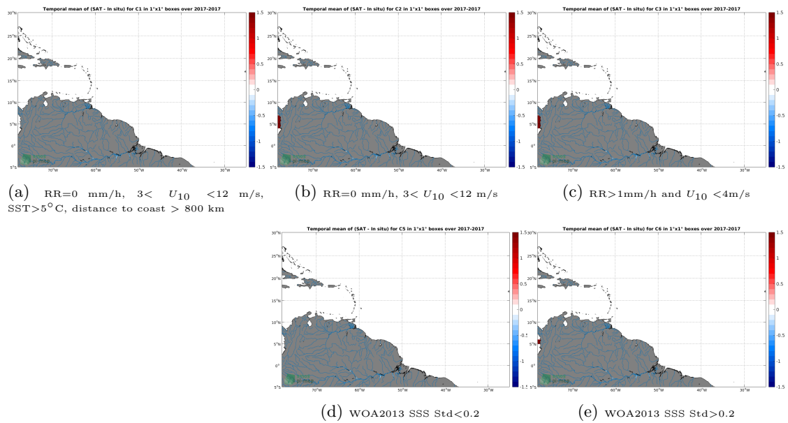
Figure 11: Temporal mean gridded over spatial boxes of size 1^\circ \times 1^\circ of \Delta SSS (SMAP-L3-RSS-V4-8DAY-RUNNING - Surface drifters) for 5 different subdatasets corresponding to: RR=0 mm/h, 3 < U_{10} < 12 m/s, SST > 5^\circ C , distance to coast > 800 km (a), RR=0 mm/h, 3 < U_{10} < 12 m/s (b), RR > 1 mm/h and U_{10} < 4 m/s (c), WOA2013 SSS Std < 0.2 (d), WOA2013 SSS Std > 0.2 (e).
