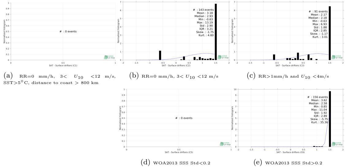
Figure 12: Normalized histogram of \Delta\text{SSS} (SMAP-L3-RSS-V4-8DAY-RUNNING - Surface drifters) for 5 different subdatasets corresponding to: RR=0 mm/h, 3 < U_{10} < 12 m/s, SST > 5^\circ\text{C} , distance to coast > 800 km (a), RR=0 mm/h, 3 < U_{10} < 12 m/s (b), RR > 1\text{mm/h} and U_{10} < 4\text{m/s} (c), WOA2013 SSS Std < 0.2 (d), WOA2013 SSS Std > 0.2 (e).
