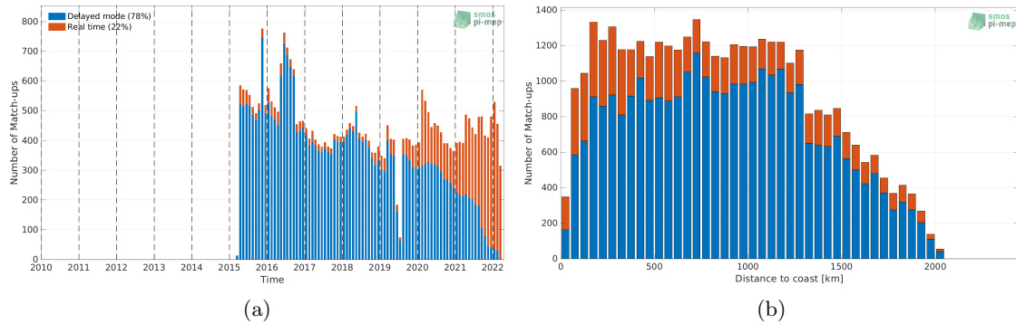
Figure 1: Number of match-ups between Argo and SMAP SSS L3 v4 - 8-Day running (RSS) SSS as a function of time (a) and as function of the distance to coast (b) over the Amazon and Orinoco river plumes Pi-MEP region and for the full satellite product period.
