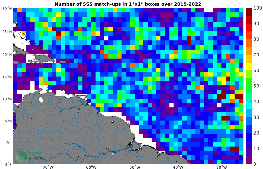
Figure 4: Number of SSS match-ups between Argo SSS and the SMAP SSS L3 v4 - 8-Day running (RSS) SSS product for the Amazon and Orinoco river plumes Pi-MEP region over 1^\circ \times 1^\circ boxes and for the full satellite product period.
