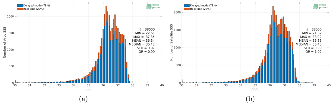
Figure 2: Histograms of SSS from Argo (a) and SMAP SSS L3 v4 - 8-Day running (RSS) (b) considering all match-up pairs per bins of 0.1 over the Amazon and Orinoco river plumes Pi-MEP region and for the full satellite product period.
