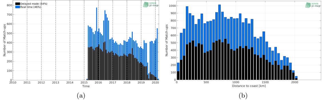
Figure 1: Number of match-ups between Argo and SMAP-L3-RSS-V4-8DAY-RUNNING SSS as a function of time (a) and as function of the distance to coast (b) over the Amazon and Orinoco river plumes Pi-MEP region and for the full satellite product period.
