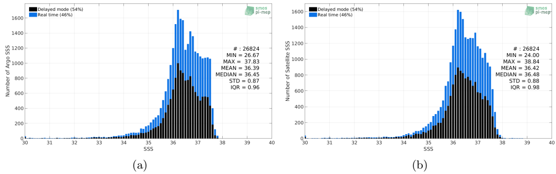
Figure 2: Histograms of SSS from Argo (a) and SMAP-L3-RSS-V4-8DAY-RUNNING (b) considering all match-up pairs per bins of 0.1 over the Amazon and Orinoco river plumes Pi-MEP region and for the full satellite product period.
