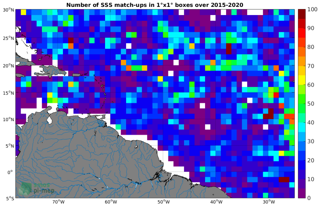
Figure 4: Number of SSS match-ups between Argos SSS and the SMAP-L3-RSS-V4-8DAY-RUNNING SSS product for the Amazon and Orinoco river plumes Pi-MEP region over 1°x1° boxes and for the full satellite product period.
