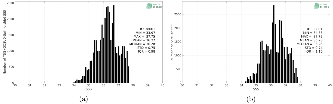
Figure 2: Histograms of SSS from TSG (GOSUD-Sailing-ship) (a) and SMAP SSS L3 v4 - Monthly (RSS) (b) considering all match-up pairs per bins of 0.1 over the Amazon and Orinoco river plumes Pi-MEP region and for the full satellite product period.
