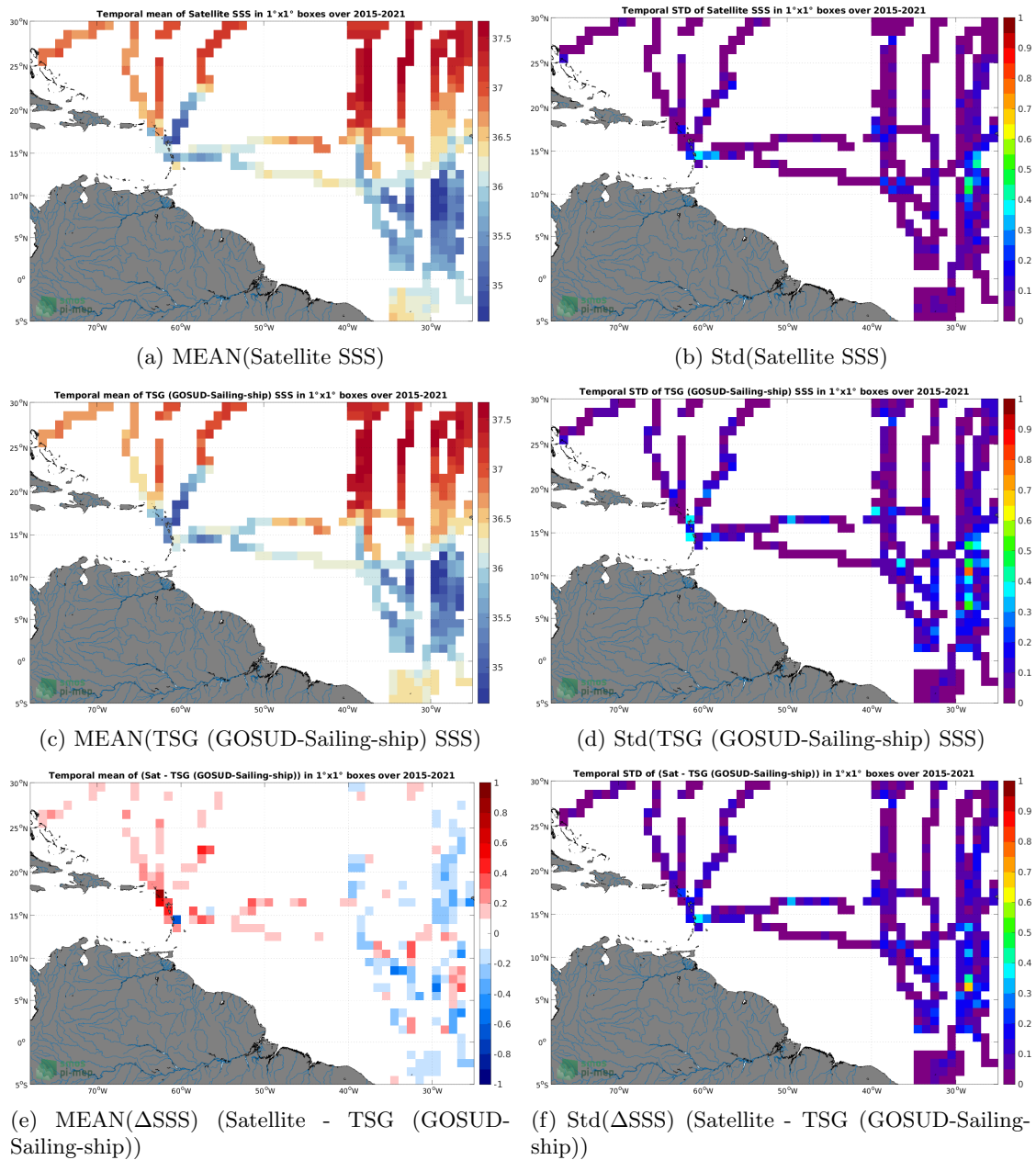
Figure 6: Temporal mean (left) and Std (right) of SSS from SMAP SSS L3 v4 - Monthly (RSS) (top), TSG (GOSUD-Sailing-ship) (middle), and of \Delta SSS (Satellite - TSG (GOSUD-Sailing-ship)). Only match-up pairs are used to generate these maps.
