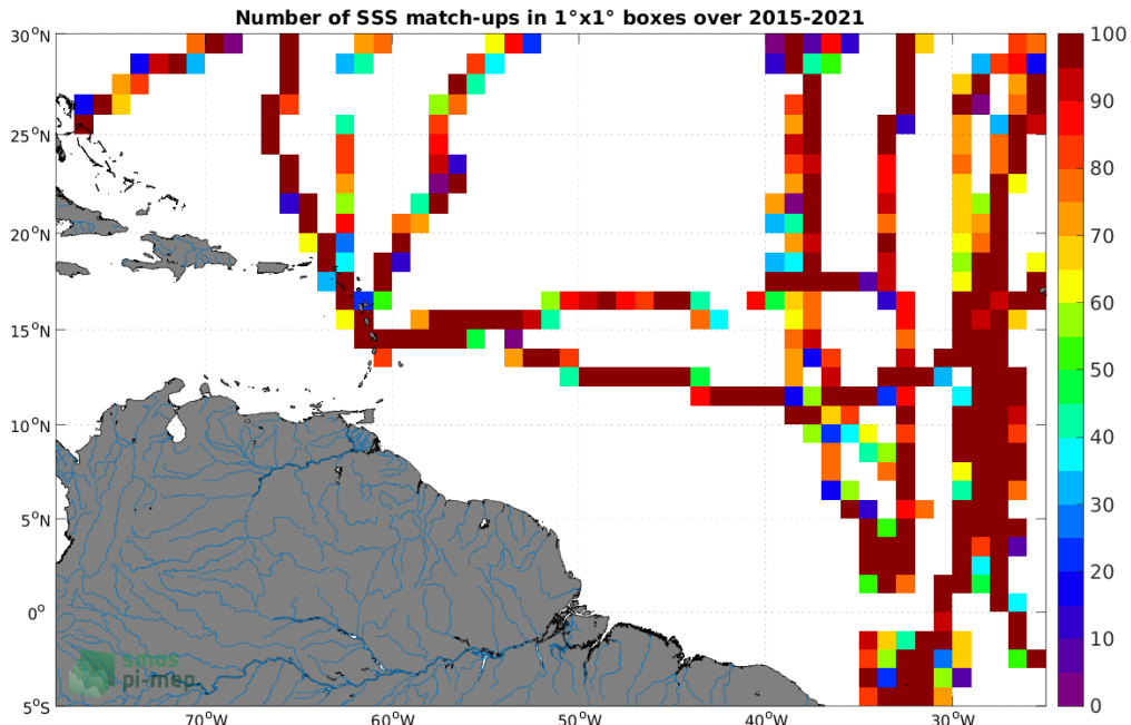
Figure 4: Number of SSS match-ups between TSG (GOSUD-Sailing-ship) SSS and the SMAP SSS L3 v4 - Monthly (RSS) SSS product for the Amazon and Orinoco river plumes Pi-MEP region over 1^\circ \times 1^\circ boxes and for the full satellite product period.
