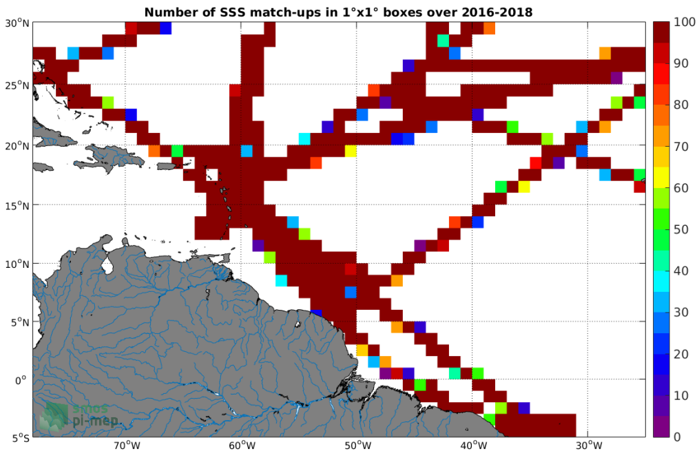
Figure 4: Number of SSS match-ups between TSG-GOSUD-Research-vessel SSS and the SMAP-L3-RSS-V4-MONTHLY SSS product for the Amazon and Orinoco river plumes Pi-MEP region over 1°x1° boxes and for the full satellite product period.
