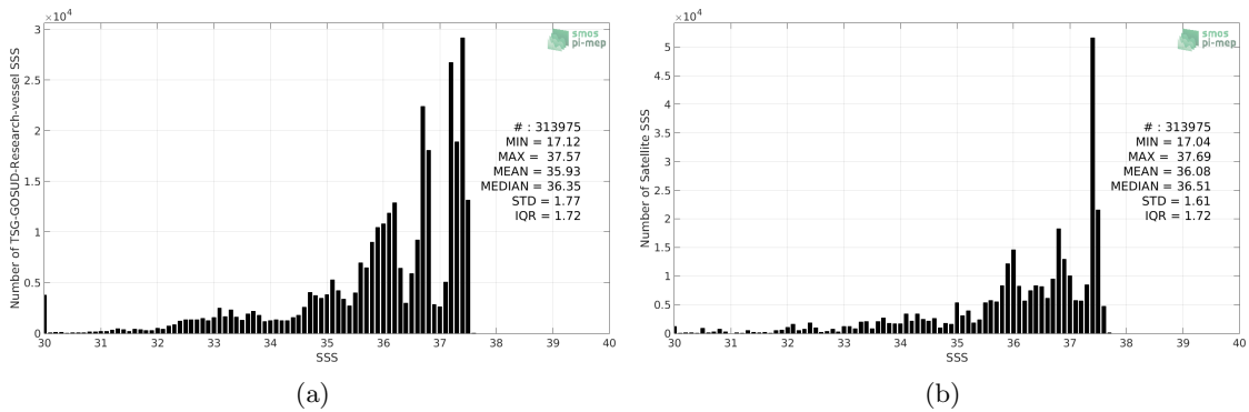
Figure 2: Histograms of SSS from TSG-GOSUD-Research-vessel (a) and SMAP-L3-RSS-V4-MONTHLY (b) considering all match-up pairs per bins of 0.1 over the Amazo and Orinoco river plumes Pi-MEP region and for the full satellite product period.
