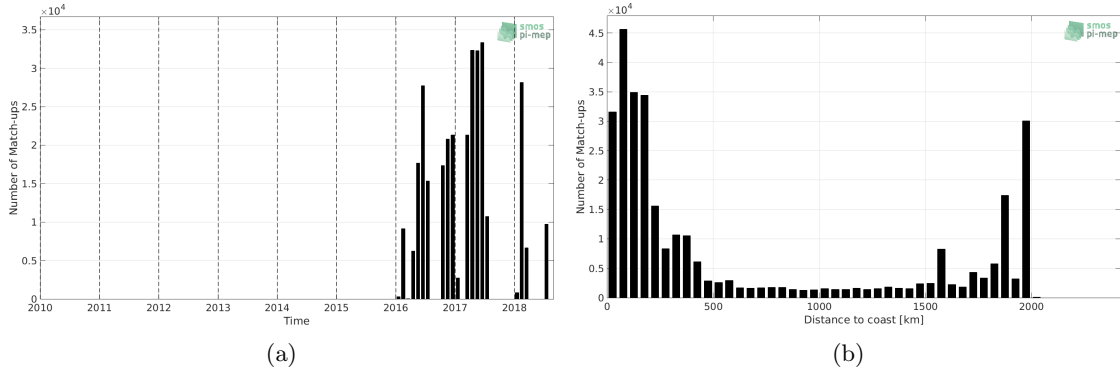
Figure 1: Number of match-ups between TSG-GOSUD-Research-vessel and SMAP-L3-RSS-V4-MONTHLY SSS as a function of time (a) and as function of the distance to coast (b) over the Amazon and Orinoco river plumes Pi-MEP region and for the full satellite product period.
