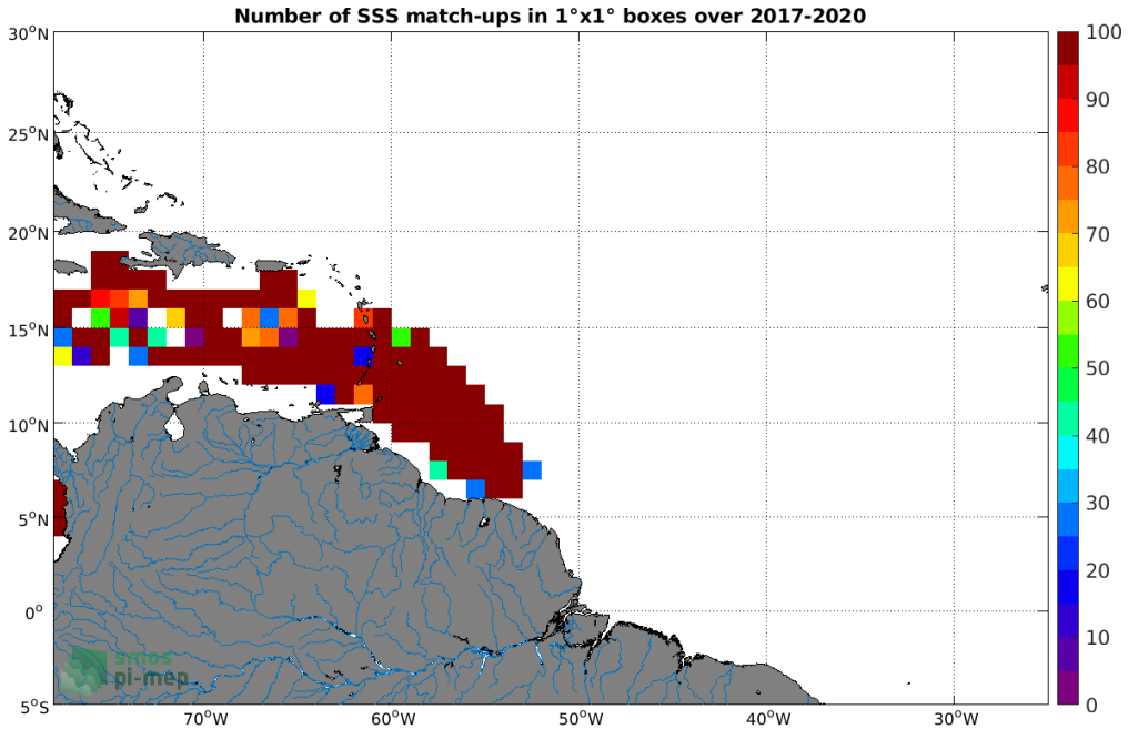
Figure 3: Number of SSS match-ups between Surface drifters SSS and the SMAP SSS L3 v4 - Monthly (RSS) SSS product for the Amazon and Orinoco river plumes Pi-MEP region over 1° × 1° boxes and for the full satellite product period.
