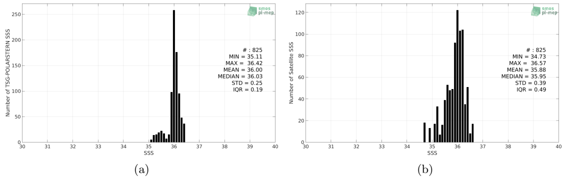
Figure 2: Histograms of SSS from TSG-POLARSTERN (a) and SMAP-L3-RSS-V3-8DAY-RUNNING-70KM (b) considering all match-up pairs per bins of 0.1 over the Amazon and Orinoco river plumes Pi-MEP region and for the full satellite product period.
