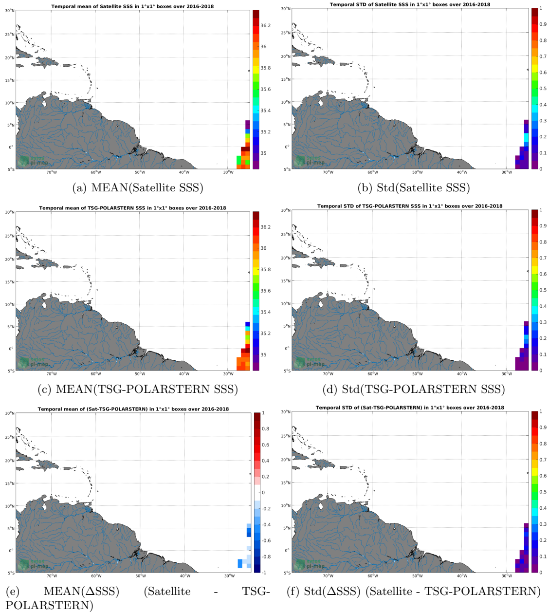
Figure 6: Temporal mean (left) and Std (right) of SSS from SMAP-L3-RSS-V3-8DAY-RUNNING-70KM (top), TSG-POLARSTERN (middle), and of \Delta SSS (Satellite - TSG-POLARSTERN). Only match-up pairs are used to generate these maps.
