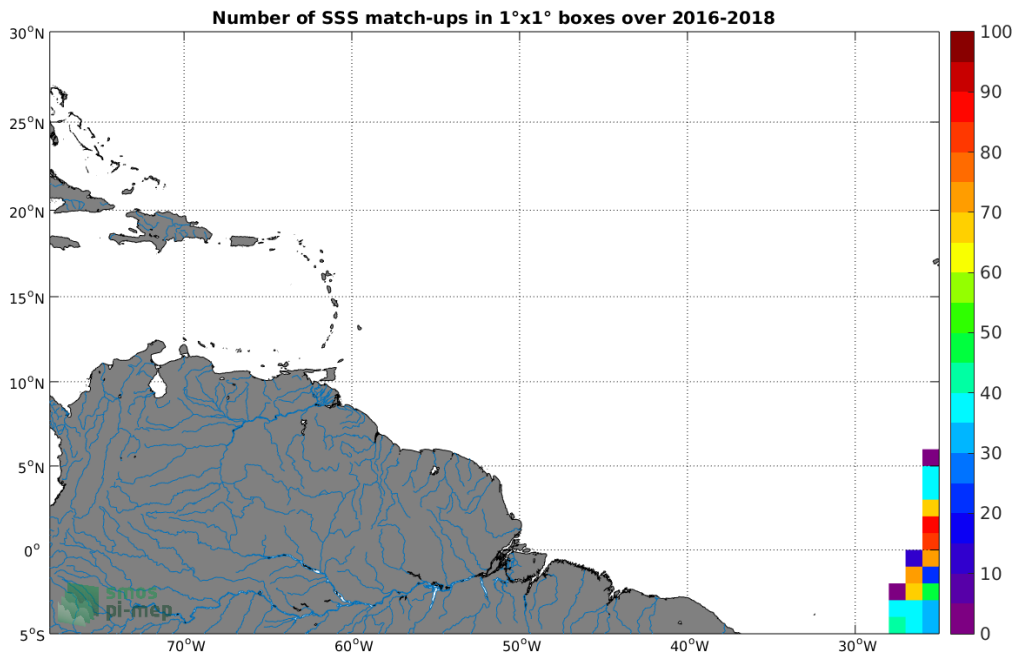
Figure 4: Number of SSS match-ups between TSG-POLARSTERN SSS and the SMAP-L3-RSS-V3-8DAY-RUNNING-70KM SSS product for the Amazon and Orinoco river plumes Pi-MEP region over 1^\circ \times 1^\circ boxes and for the full satellite product period.
