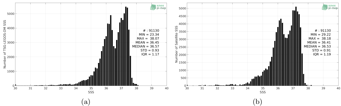
Figure 2: Histograms of SSS from TSG-LEGOS-DM (a) and SMAP-L3-RSS-V3-8DAY-RUNNING-70KM (b) considering all match-up pairs per bins of 0.1 over the Amazon and Orinoco river plumes Pi-MEP region and for the full satellite product period.
