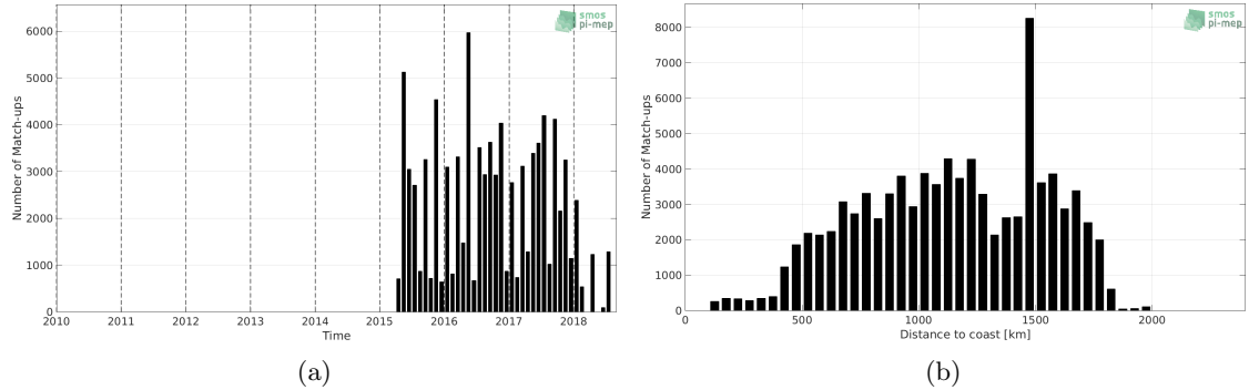
Figure 1: Number of match-ups between TSG-LEGOS-DM and SMAP-L3-RSS-V3-8DAY-RUNNING-70KM SSS as a function of time (a) and as function of the distance to coast (b) over the Amazon and Orinoco river plumes Pi-MEP region and for the full satellite product period.
