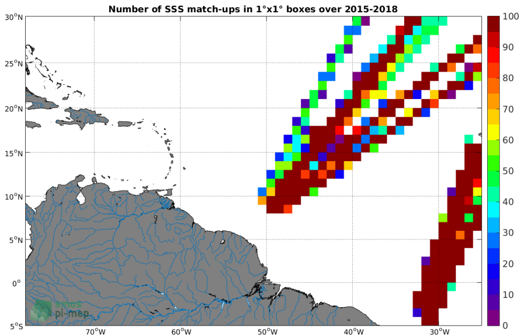
Figure 4: Number of SSS match-ups between TSG-LEGOS-DM SSS and the SMAP-L3-RSS-V3-8DAY-RUNNING-70KM SSS product for the Amazon and Orinoco river plumes Pi-MEP region over 1^\circ \times 1^\circ boxes and for the full satellite product period.
