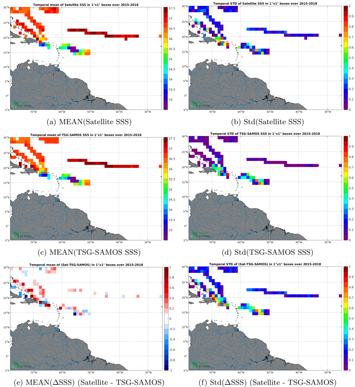
Figure 6: Temporal mean (left) and Std (right) of SSS from SMAP-L3-RSS-V3-8DAY-RUNNING-40KM (top), TSG-SAMOS (middle), and of \Delta SSS (Satellite - TSG-SAMOS). Only match-up pairs are used to generate these maps.
