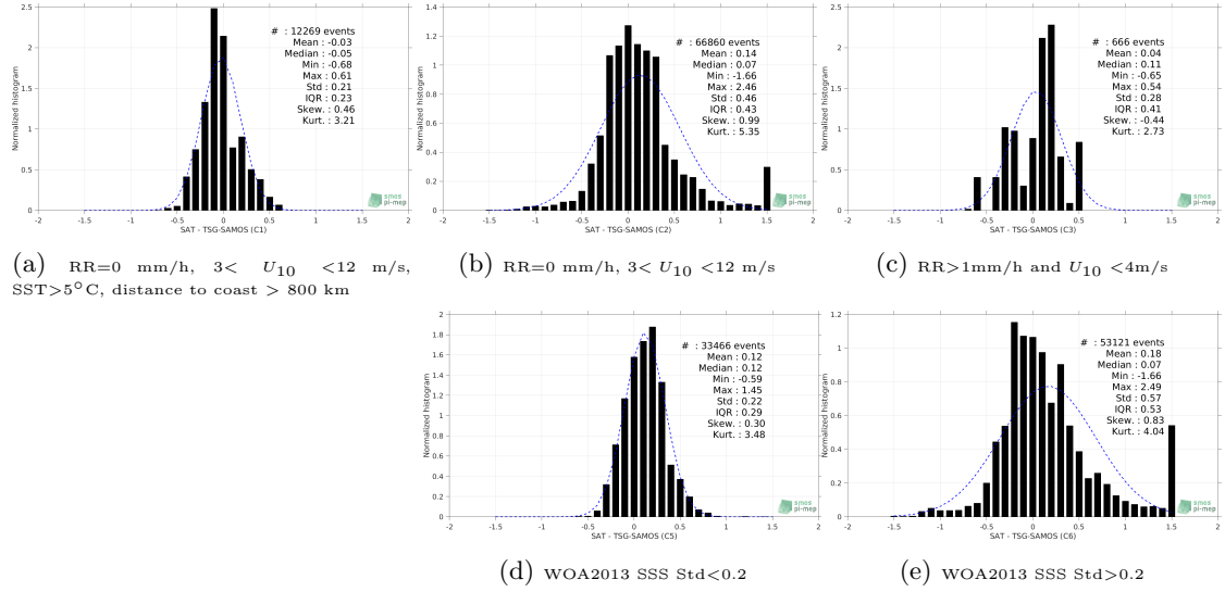
Figure 13: Normalized histogram of \Delta SSS (SMAP-L3-RSS-V3-8DAY-RUNNING-40KM - TSG-SAMOS) for 5 different subdatasets corresponding to: RR=0 mm/h, 3 < U_{10} < 12 m/s, SST > 5°C, distance to coast > 800 km (a), RR=0 mm/h, 3 < U_{10} < 12 m/s (b), RR > 1mm/h and U_{10} < 4 m/s (c), WOA2013 SSS Std < 0.2 (d), WOA2013 SSS Std > 0.2 (e).
