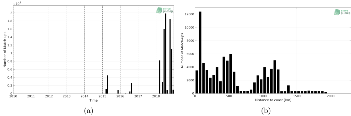
Figure 1: Number of match-ups between TSG-SAMOS and SMAP-L3-RSS-V3-8DAY-RUNNING-40KM SSS as a function of time (a) and as function of the distance to coast (b) over the Amazon and Orinoco river plumes Pi-MEP region and for the full satellite product period.
