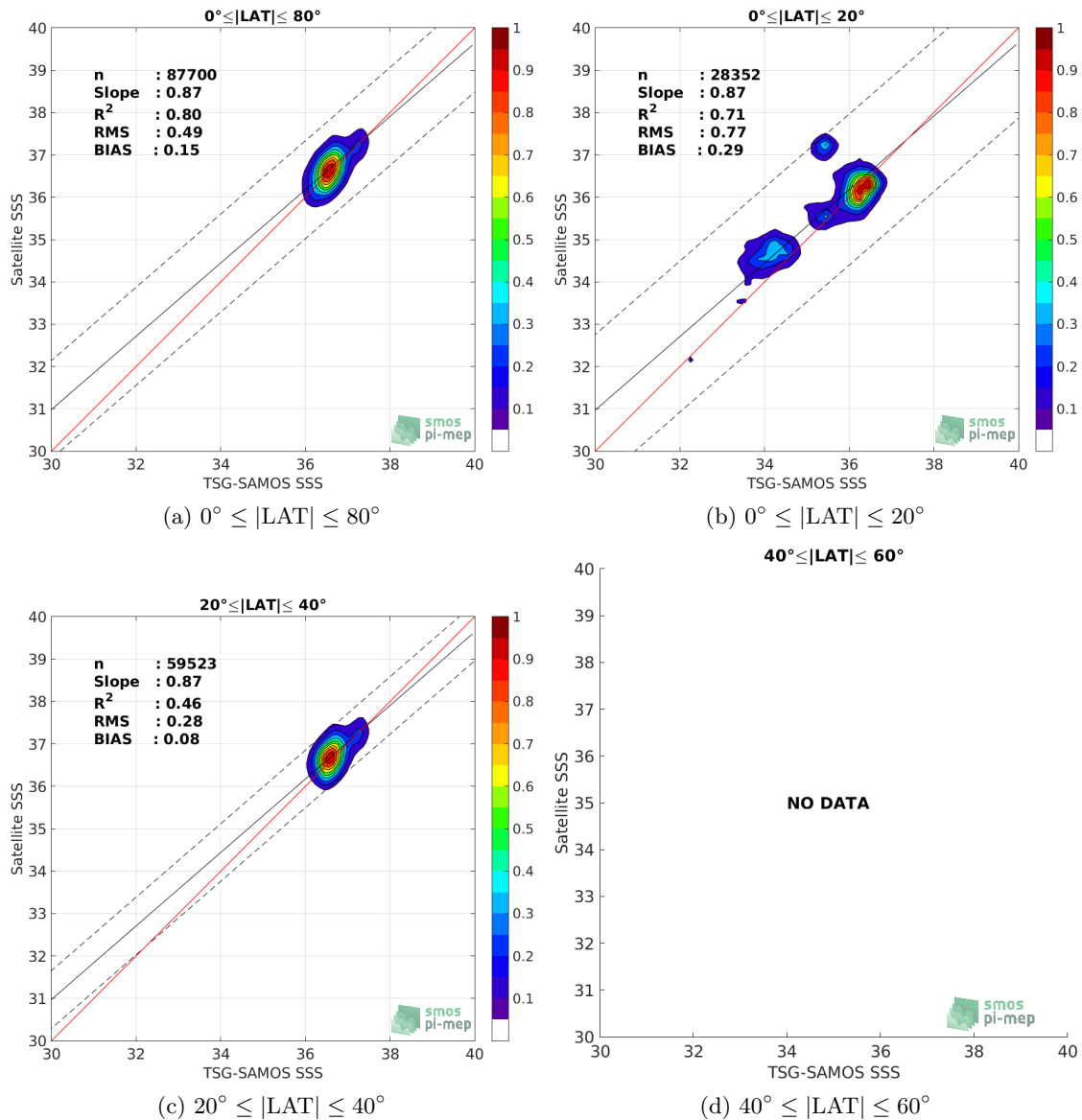
Figure 9: Contour maps of the concentration of SMAP-L3-RSS-V3-8DAY-RUNNING-40KM SSS (y-axis) versus TSG-SAMOS SSS (x-axis) at match-up pairs for different latitude bands. For each plot, the red line shows x=y . The black thin and dashed lines indicate a linear fit through the data cloud and the \pm 95\% confidence levels, respectively. The number match-up pairs n , the slope and R^2 coefficient of the linear fit, the root mean square (RMS) and the mean bias between satellite and in situ data are indicated for each latitude band in each plots.
