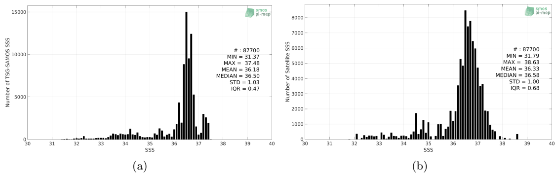
Figure 2: Histograms of SSS from TSG-SAMOS (a) and SMAP-L3-RSS-V3-8DAY-RUNNING-40KM (b) considering all match-up pairs per bins of 0.1 over the Amazon and Orinoco river plumes Pi-MEP region and for the full satellite product period.
