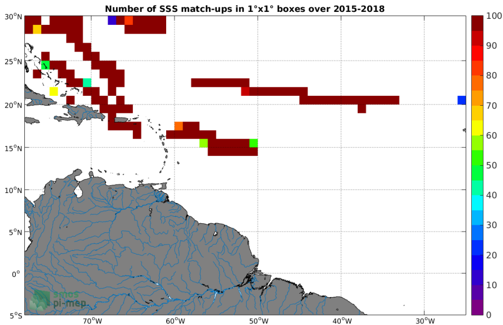
Figure 4: Number of SSS match-ups between TSG-SAMOS SSS and the SMAP-L3-RSS-V3-8DAY-RUNNING-40KM SSS product for the Amazon and Orinoco river plumes Pi-MEP region over 1^\circ \times 1^\circ boxes and for the full satellite product period.
