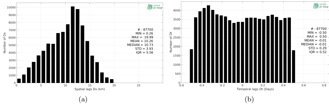
Figure 5: Histograms of the spatial (a) and temporal (b) lags between the time of the TSG-SAMOS measurements and the date of the corresponding SMAP-L3-RSS-V3-8DAY-RUNNING-40KM SSS product.
