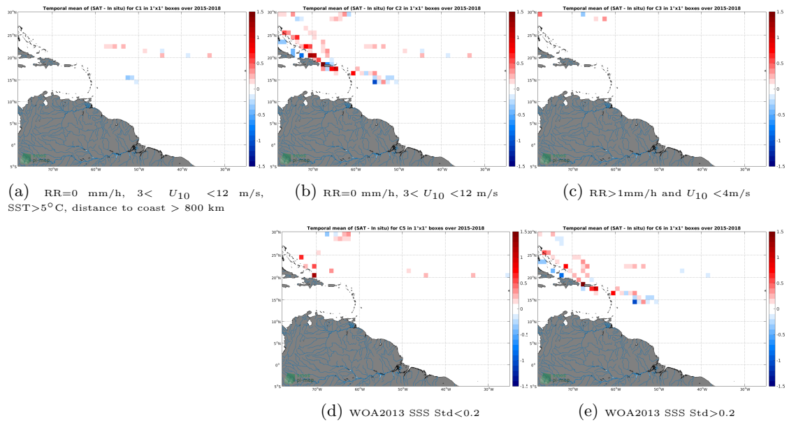
Figure 12: Temporal mean gridded over spatial boxes of size 1^\circ \times 1^\circ of \Delta SSS (SMAP-L3-RSS-V3-8DAY-RUNNING-40KM - TSG-SAMOS) for 5 different subdatasets corresponding to:RR=0 mm/h, 3 < U_{10} < 12 m/s, SST >5^\circ\text{C} , distance to coast > 800 km (a), RR=0 mm/h, 3 < U_{10} < 12 m/s (b), RR >1 mm/h and U_{10} < 4 m/s (c), WOA2013 SSS Std <0.2 (d), WOA2013 SSS Std >0.2 (e).
