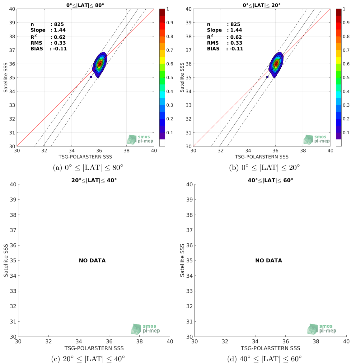
Figure 9: Contour maps of the concentration of SMAP-L3-RSS-V3-8DAY-RUNNING-40KM SSS (y-axis) versus TSG-POLARSTERN SSS (x-axis) at match-up pairs for different latitude bands. For each plot, the red line shows x=y . The black thin and dashed lines indicate a linear fit through the data cloud and the \pm 95\% confidence levels, respectively. The number match-up pairs n , the slope and R^2 coefficient of the linear fit, the root mean square (RMS) and the mean bias between satellite and in situ data are indicated for each latitude band in each plots.
