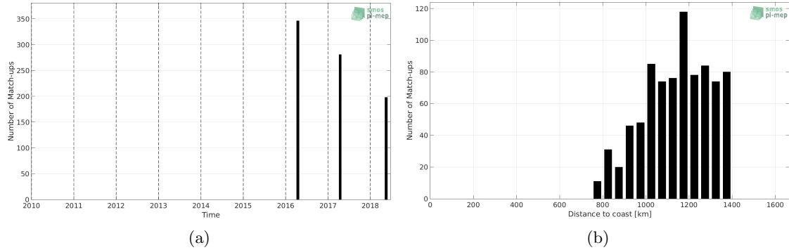
Figure 1: Number of match-ups between TSG-POLARSTERN and SMAP-L3-RSS-V3-8DAY-RUNNING-40KM SSS as a function of time (a) and as function of the distance to coast (b) over the Amazon and Orinoco river plumes Pi-MEP region and for the full satellite product period.
