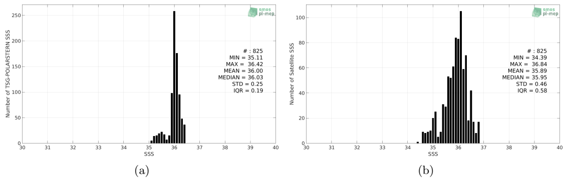
Figure 2: Histograms of SSS from TSG-POLARSTERN (a) and SMAP-L3-RSS-V3-8DAY-RUNNING-40KM (b) considering all match-up pairs per bins of 0.1 over the Amazon and Orinoco river plumes Pi-MEP region and for the full satellite product period.
